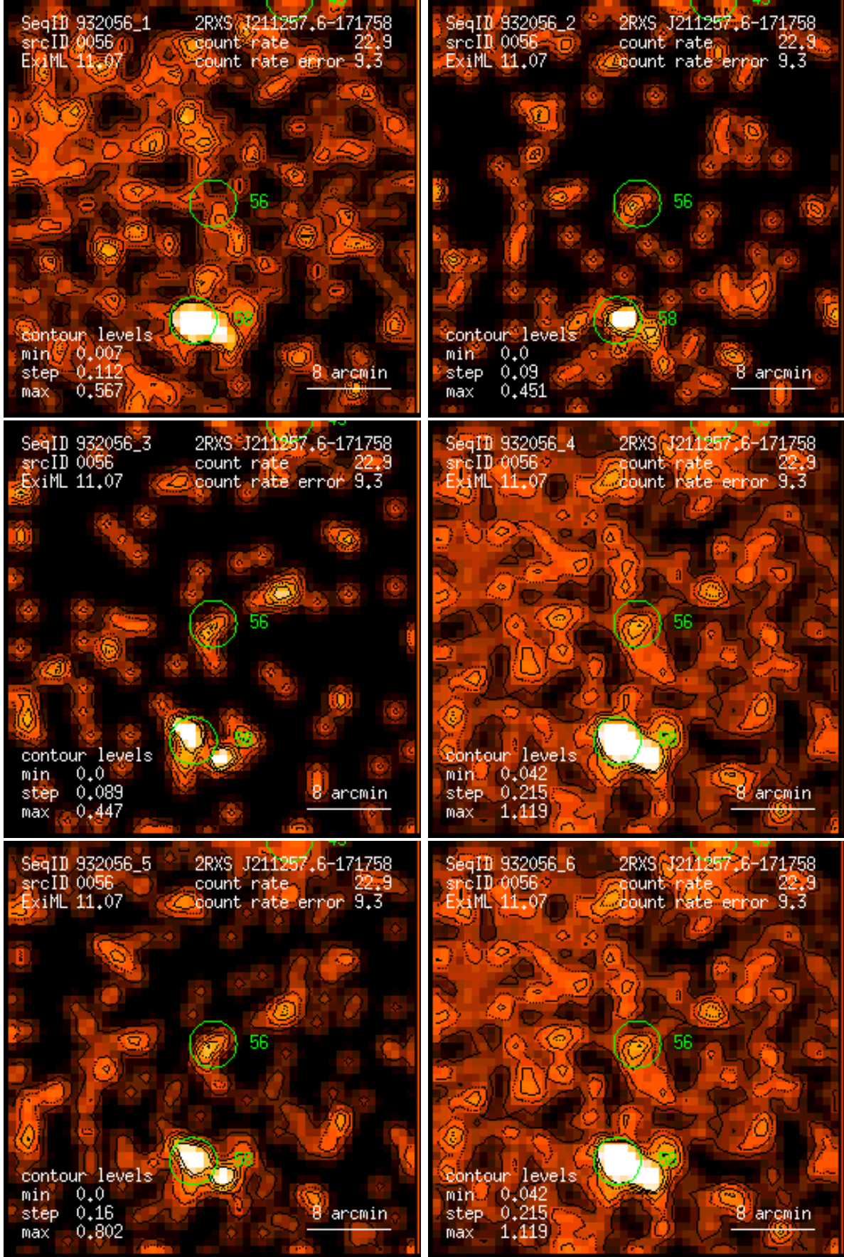
Figure 56: RASS 932056: detection 0056: band rate images, Gaussian filter: (1) PSPC channels 11 – 41, (2) 52 – 90, (3) 91 – 201, (4) 11 – 235, (5) 52 – 201, (6) 11 – 201. Broad band rates in counts/ks. Band rate contour levels in counts/ks/arcmin 2 .
