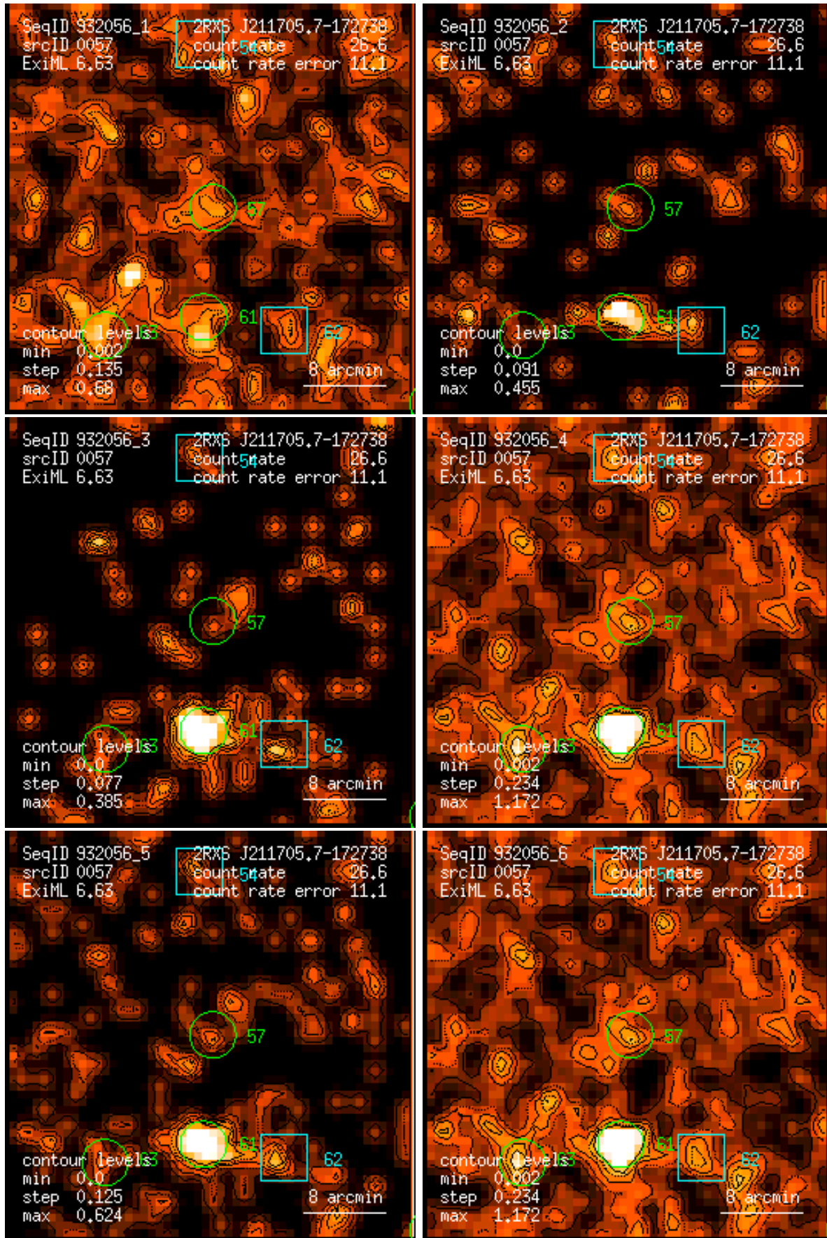
Figure 57: RASS 932056: detection 0057: band rate images, Gaussian filter: (1) PSPC channels 11 – 41, (2) 52 – 90, (3) 91 – 201, (4) 11 – 235, (5) 52 – 201, (6) 11 – 201. Broad band rates in counts/ks. Band rate contour levels in counts/ks/arcmin 2 .
