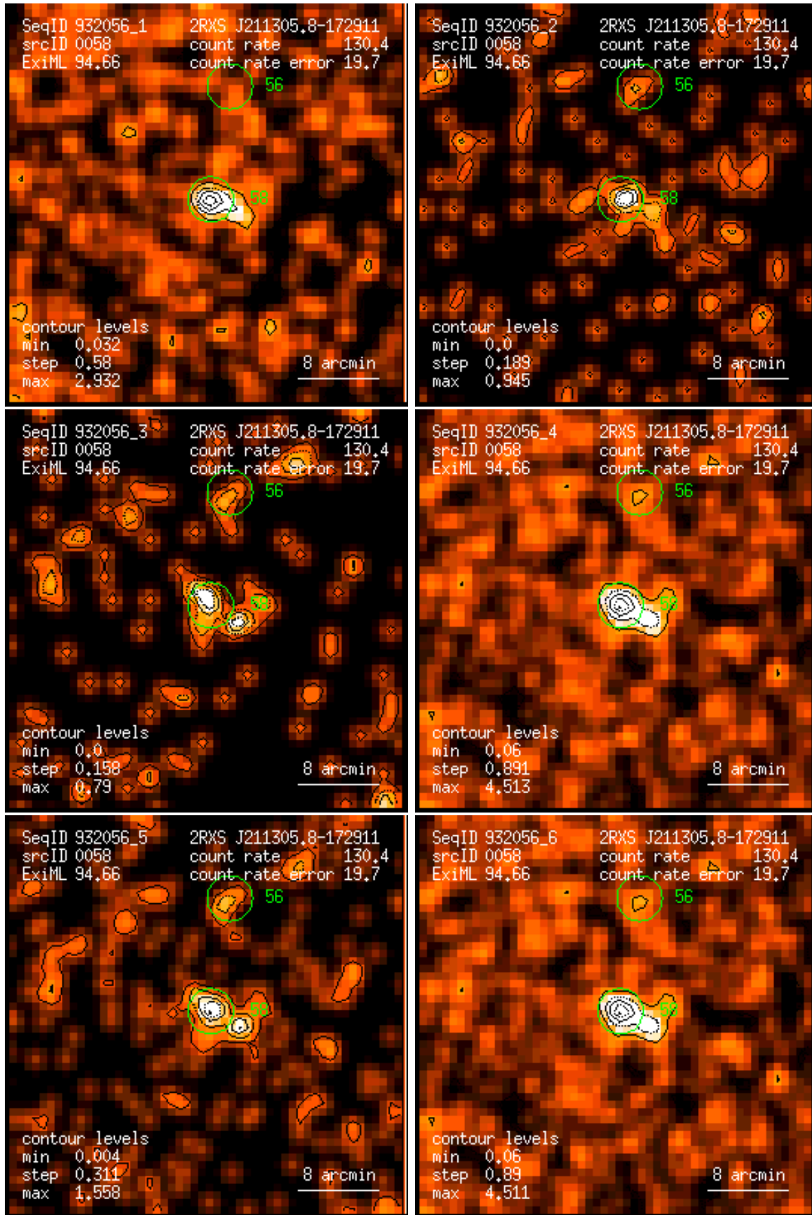
Figure 58: RASS 932056: detection 0058: band rate images, Gaussian filter: (1) PSPC channels 11 – 41, (2) 52 – 90, (3) 91 – 201, (4) 11 – 235, (5) 52 – 201, (6) 11 – 201. Broad band rates in counts/ks. Band rate contour levels in counts/ks/arcmin 2 .
