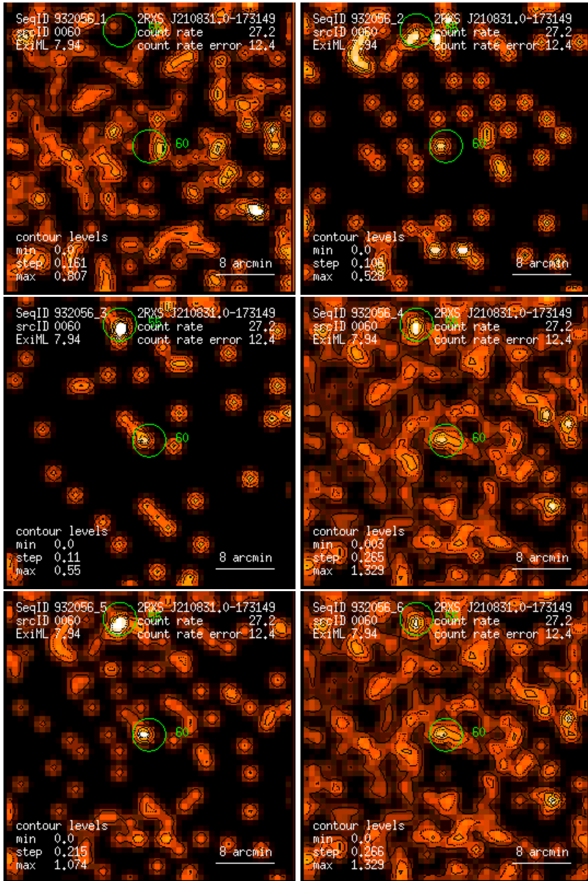
Figure 60: RASS 932056: detection 0060: band rate images, Gaussian filter: (1) PSPC channels 11 – 41, (2) 52 – 90, (3) 91 – 201, (4) 11 – 235, (5) 52 – 201, (6) 11 – 201. Broad band rates in counts/ks. Band rate contour levels in counts/ks/arcmin 2 .
