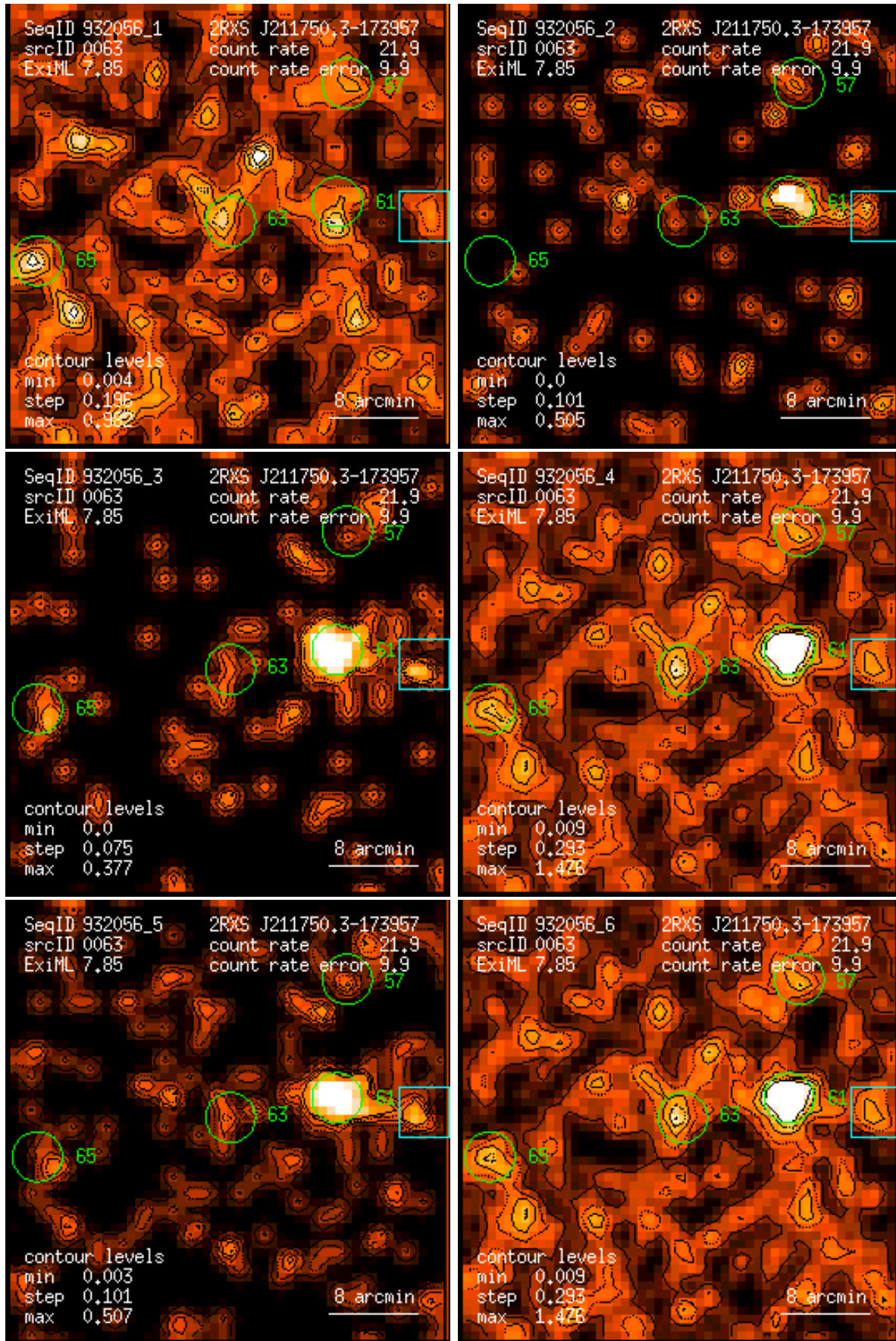
Figure 63: RASS 932056: detection 0063: band rate images, Gaussian filter: (1) PSPC channels 11 – 41, (2) 52 – 90, (3) 91 – 201, (4) 11 – 235, (5) 52 – 201, (6) 11 – 201. Broad band rates in counts/ks. Band rate contour levels in counts/ks/arcmin 2 .
