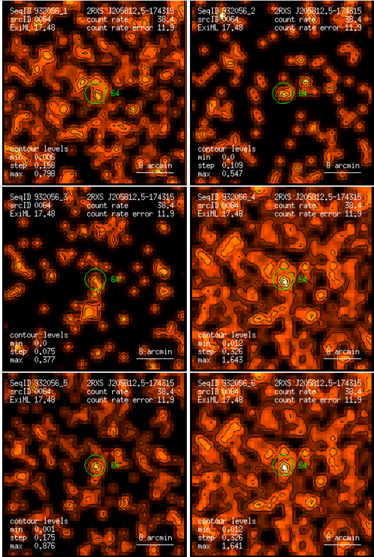
Figure 64: RASS 932056: detection 0064: band rate images, Gaussian filter: (1) PSPC channels 11 – 41, (2) 52 – 90, (3) 91 – 201, (4) 11 – 235, (5) 52 – 201, (6) 11 – 201. Broad band rates in counts/ks. Band rate contour levels in counts/ks/arcmin 2 .
