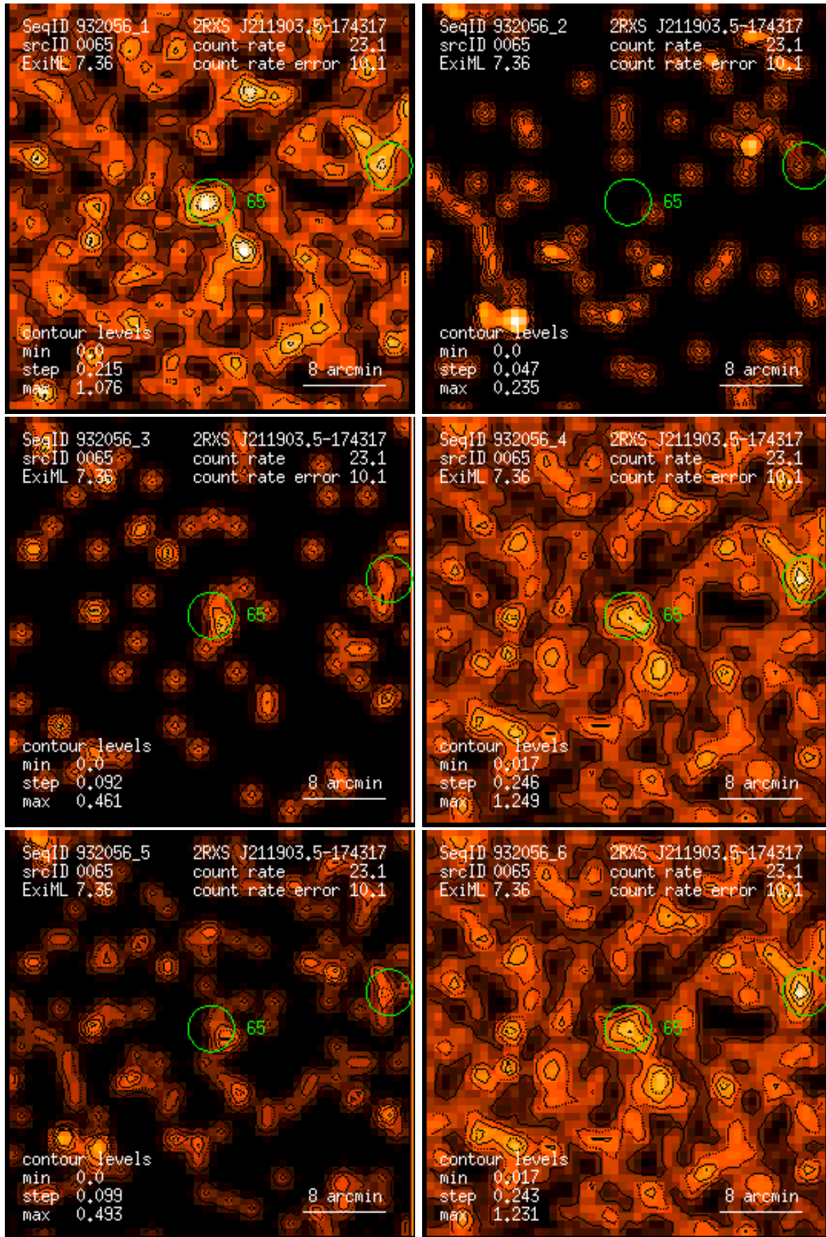
Figure 65: RASS 932056: detection 0065: band rate images, Gaussian filter: (1) PSPC channels 11 – 41, (2) 52 – 90, (3) 91 – 201, (4) 11 – 235, (5) 52 – 201, (6) 11 – 201. Broad band rates in counts/ks. Band rate contour levels in counts/ks/arcmin 2 .
