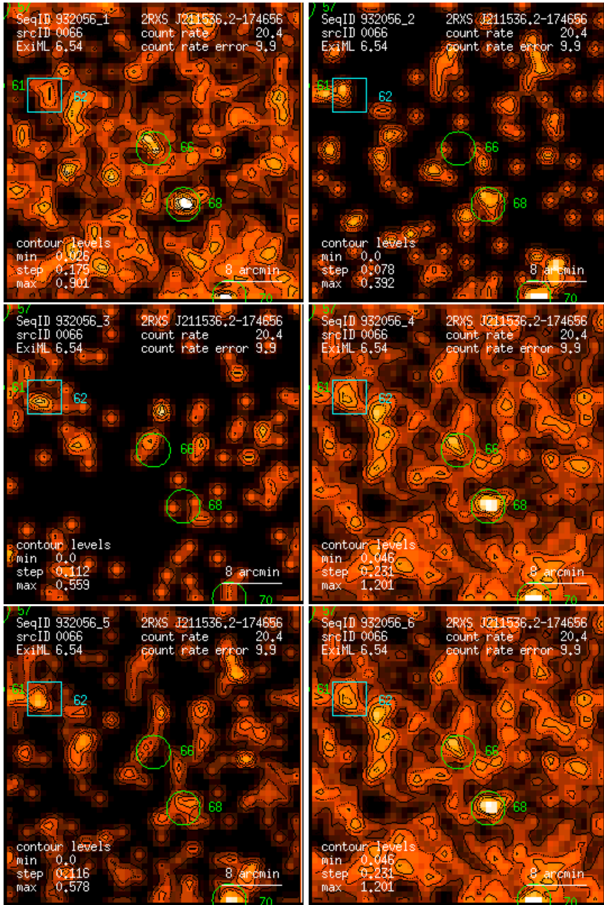
Figure 66: RASS 932056: detection 0066: band rate images, Gaussian filter: (1) PSPC channels 11 – 41, (2) 52 – 90, (3) 91 – 201, (4) 11 – 235, (5) 52 – 201, (6) 11 – 201. Broad band rates in counts/ks. Band rate contour levels in counts/ks/arcmin 2 .
