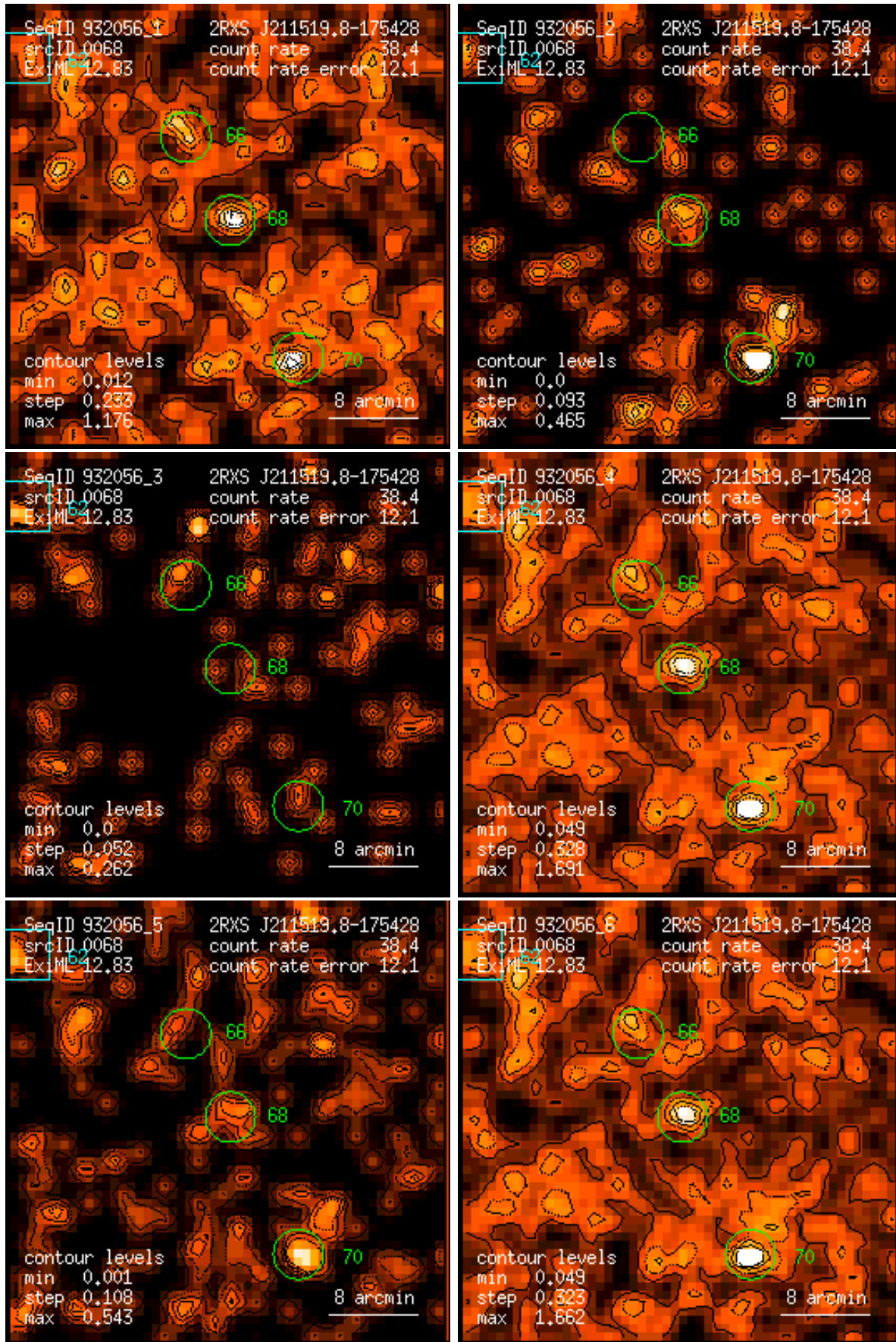
Figure 68: RASS 932056: detection 0068: band rate images, Gaussian filter: (1) PSPC channels 11 – 41, (2) 52 – 90, (3) 91 – 201, (4) 11 – 235, (5) 52 – 201, (6) 11 – 201. Broad band rates in counts/ks. Band rate contour levels in counts/ks/arcmin 2 .
