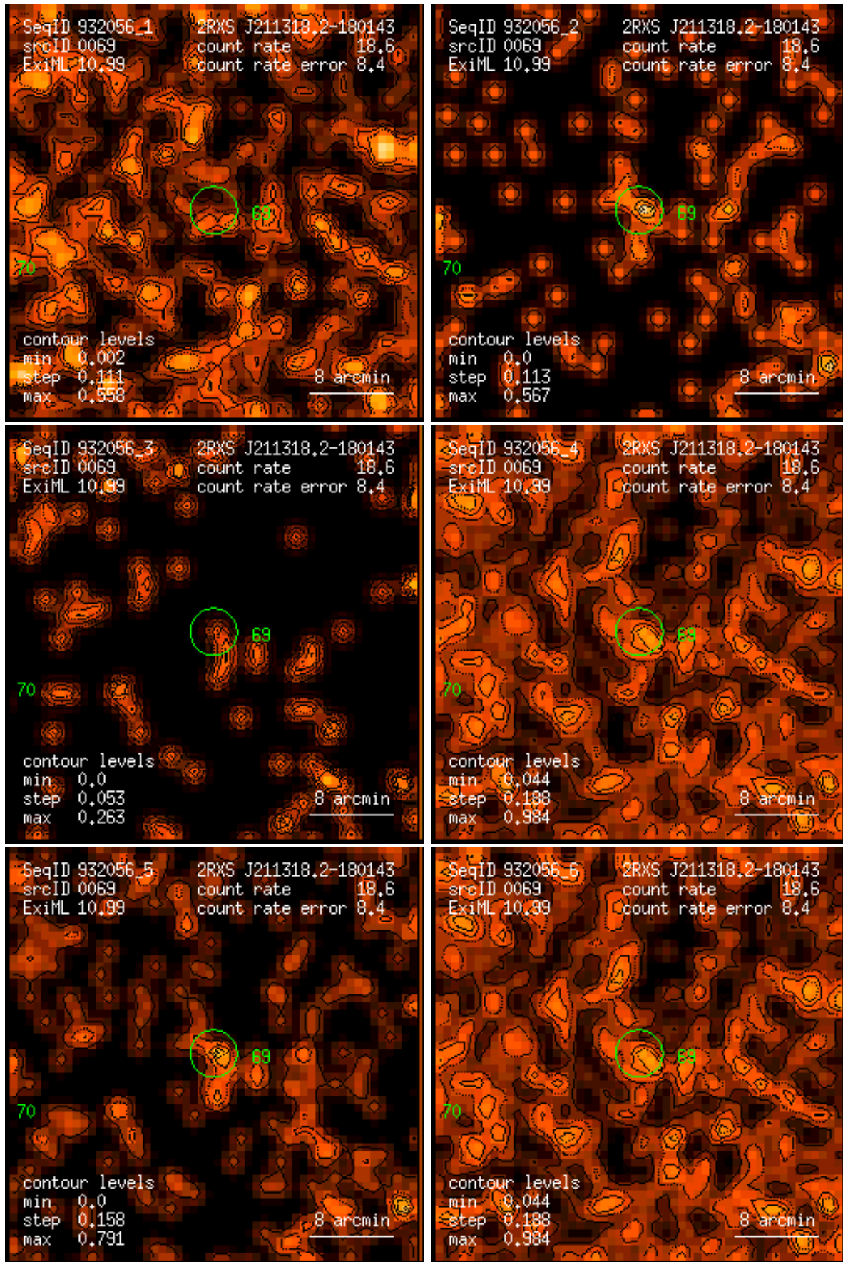
Figure 69: RASS 932056: detection 0069: band rate images, Gaussian filter: (1) PSPC channels 11 – 41, (2) 52 – 90, (3) 91 – 201, (4) 11 – 235, (5) 52 – 201, (6) 11 – 201. Broad band rates in counts/ks. Band rate contour levels in counts/ks/arcmin 2 .
