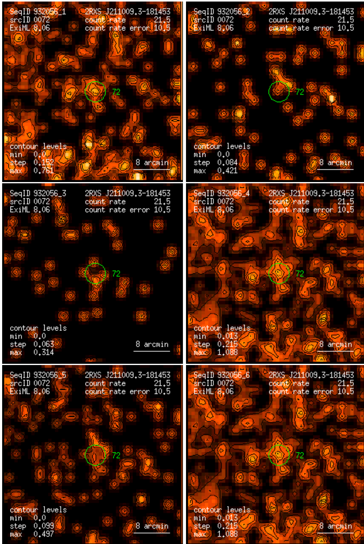
Figure 72: RASS 932056: detection 0072: band rate images, Gaussian filter: (1) PSPC channels 11 – 41, (2) 52 – 90, (3) 91 – 201, (4) 11 – 235, (5) 52 – 201, (6) 11 – 201. Broad band rates in counts/ks. Band rate contour levels in counts/ks/arcmin 2 .
