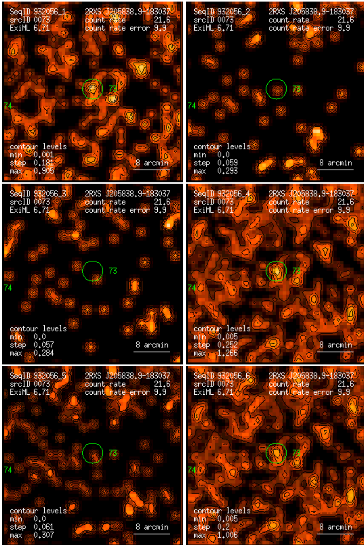
Figure 73: RASS 932056: detection 0073: band rate images, Gaussian filter: (1) PSPC channels 11 – 41, (2) 52 – 90, (3) 91 – 201, (4) 11 – 235, (5) 52 – 201, (6) 11 – 201. Broad band rates in counts/ks. Band rate contour levels in counts/ks/arcmin 2 .
