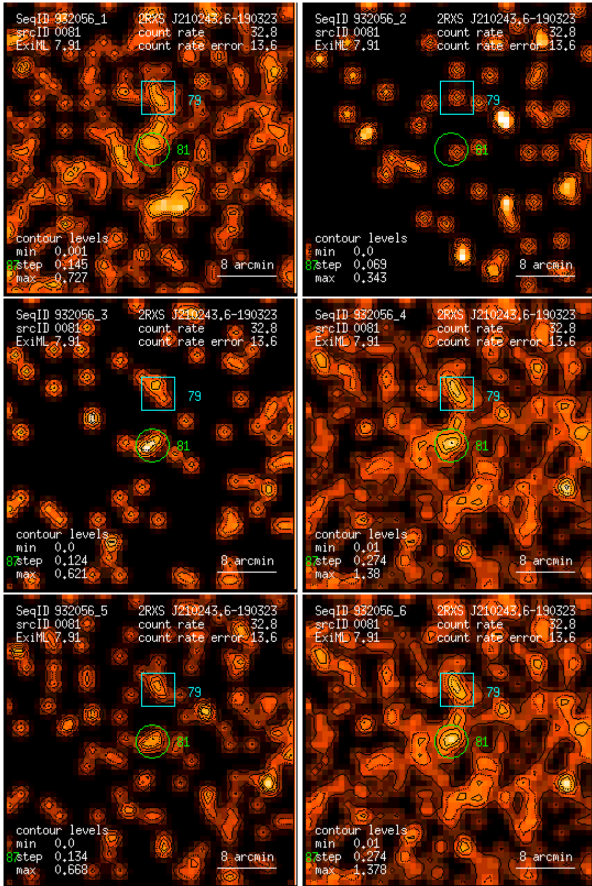
Figure 81: RASS 932056: detection 0081: band rate images, Gaussian filter: (1) PSPC channels 11 – 41, (2) 52 – 90, (3) 91 – 201, (4) 11 – 235, (5) 52 – 201, (6) 11 – 201. Broad band rates in counts/ks. Band rate contour levels in counts/ks/arcmin 2 .
