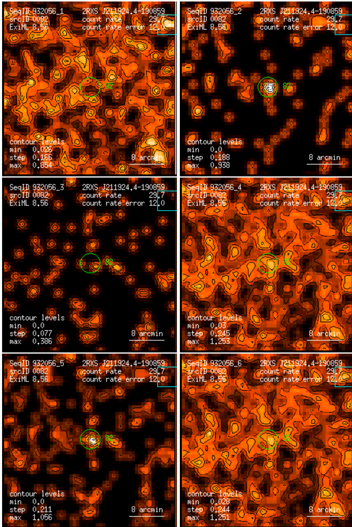
Figure 82: RASS 932056: detection 0082: band rate images, Gaussian filter: (1) PSPC channels 11 – 41, (2) 52 – 90, (3) 91 – 201, (4) 11 – 235, (5) 52 – 201, (6) 11 – 201. Broad band rates in counts/ks. Band rate contour levels in counts/ks/arcmin 2 .
