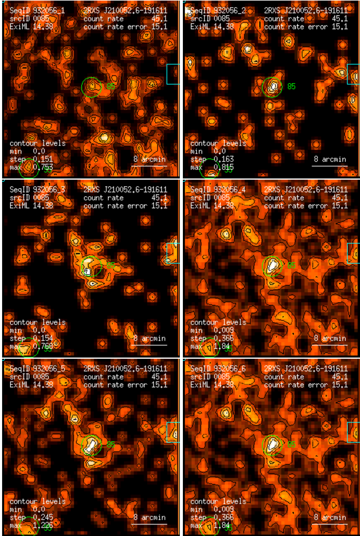
Figure 85: RASS 932056: detection 0085: band rate images, Gaussian filter: (1) PSPC channels 11 – 41, (2) 52 – 90, (3) 91 – 201, (4) 11 – 235, (5) 52 – 201, (6) 11 – 201. Broad band rates in counts/ks. Band rate contour levels in counts/ks/arcmin 2 .
