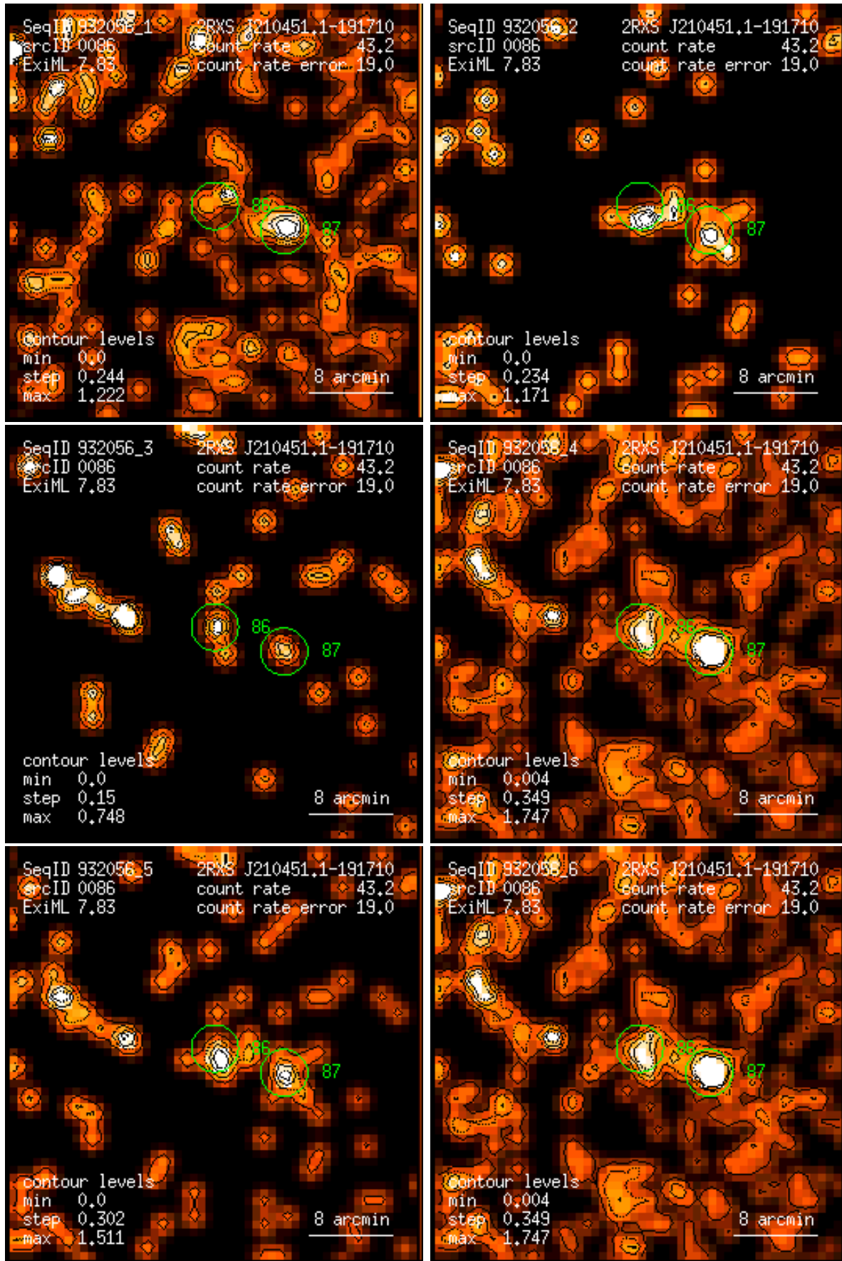
Figure 86: RASS 932056: detection 0086: band rate images, Gaussian filter: (1) PSPC channels 11 – 41, (2) 52 – 90, (3) 91 – 201, (4) 11 – 235, (5) 52 – 201, (6) 11 – 201. Broad band rates in counts/ks. Band rate contour levels in counts/ks/arcmin 2 .
