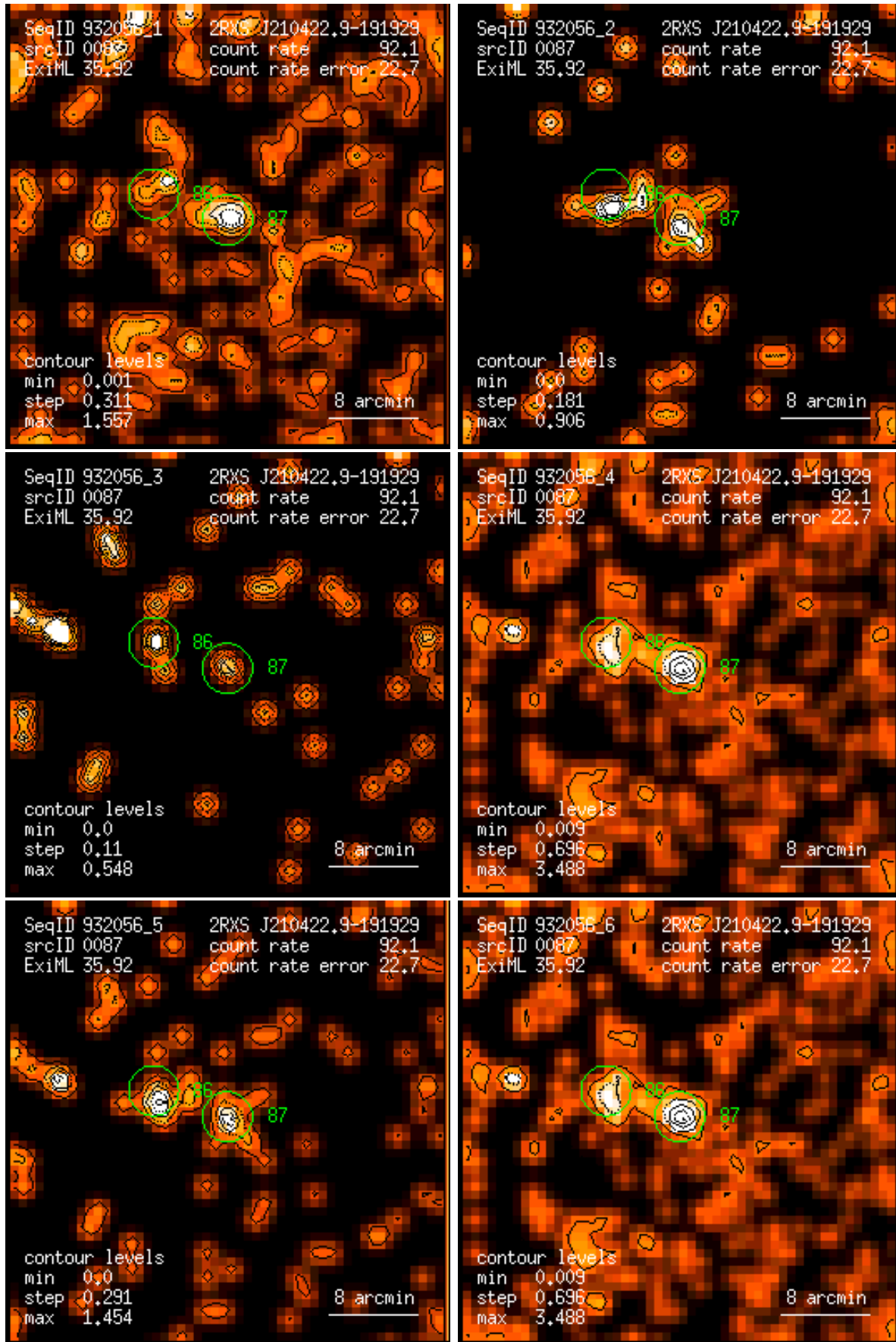
Figure 87: RASS 932056: detection 0087: band rate images, Gaussian filter: (1) PSPC channels 11 – 41, (2) 52 – 90, (3) 91 – 201, (4) 11 – 235, (5) 52 – 201, (6) 11 – 201. Broad band rates in counts/ks. Band rate contour levels in counts/ks/arcmin 2 .
