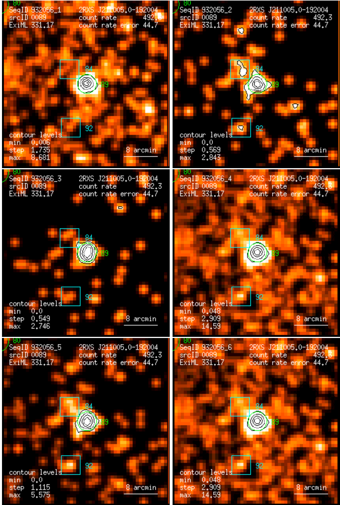
Figure 89: RASS 932056: detection 0089: band rate images, Gaussian filter: (1) PSPC channels 11 – 41, (2) 52 – 90, (3) 91 – 201, (4) 11 – 235, (5) 52 – 201, (6) 11 – 201. Broad band rates in counts/ks. Band rate contour levels in counts/ks/arcmin 2 .
