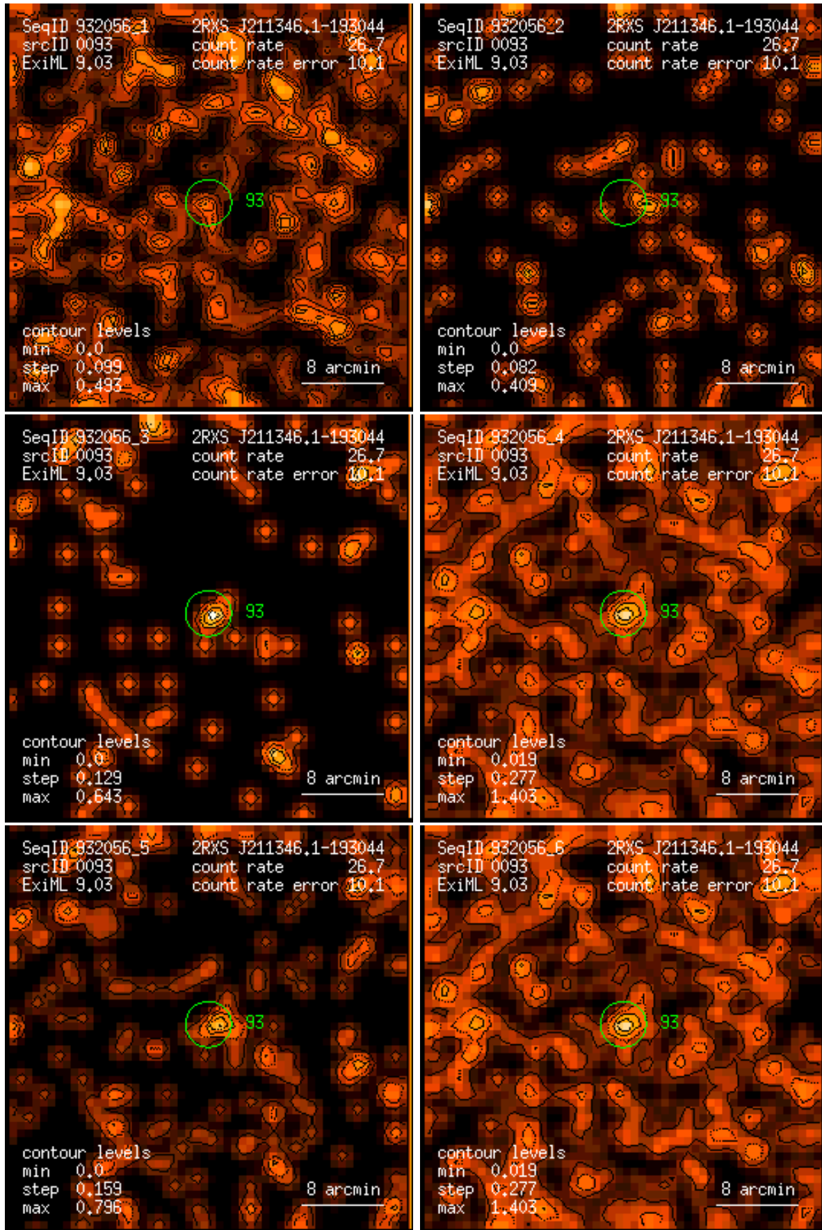
Figure 93: RASS 932056: detection 0093: band rate images, Gaussian filter: (1) PSPC channels 11 – 41, (2) 52 – 90, (3) 91 – 201, (4) 11 – 235, (5) 52 – 201, (6) 11 – 201. Broad band rates in counts/ks. Band rate contour levels in counts/ks/arcmin 2 .
