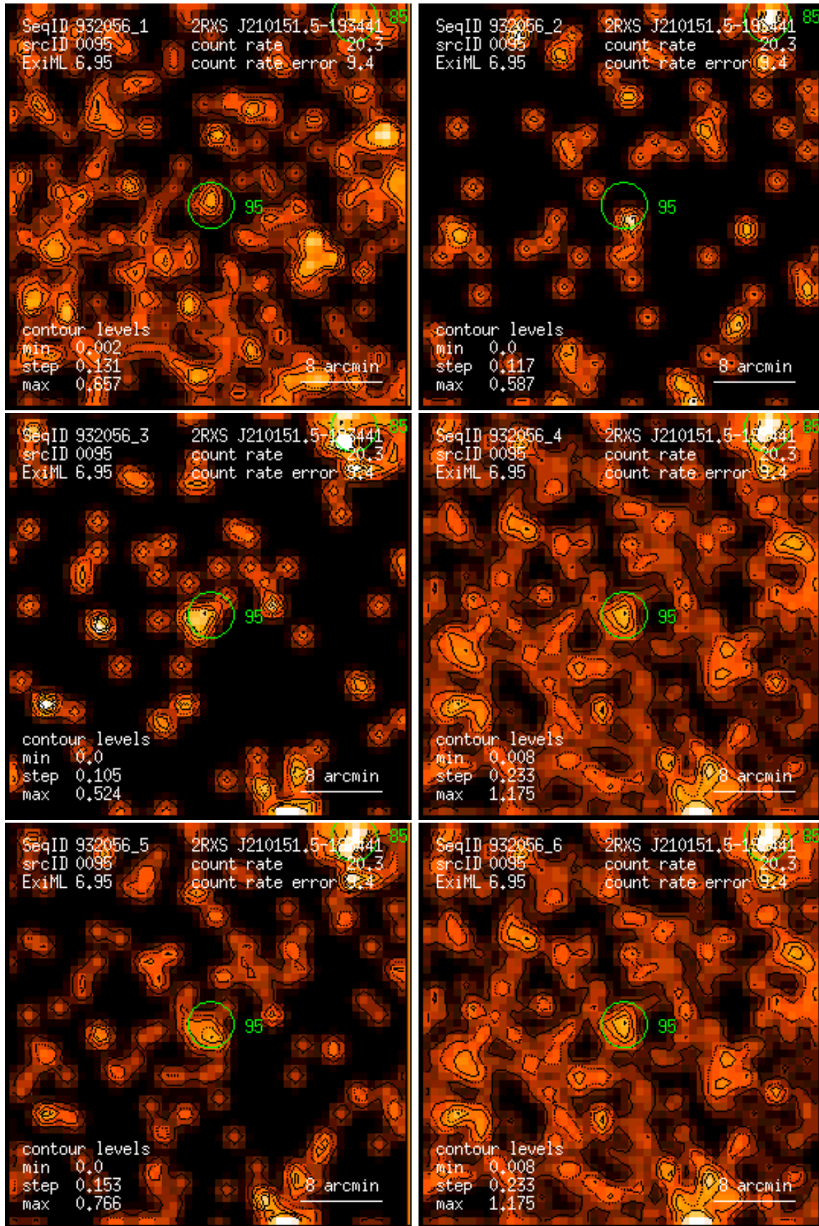
Figure 95: RASS 932056: detection 0095: band rate images, Gaussian filter: (1) PSPC channels 11 – 41, (2) 52 – 90, (3) 91 – 201, (4) 11 – 235, (5) 52 – 201, (6) 11 – 201. Broad band rates in counts/ks. Band rate contour levels in counts/ks/arcmin 2 .
