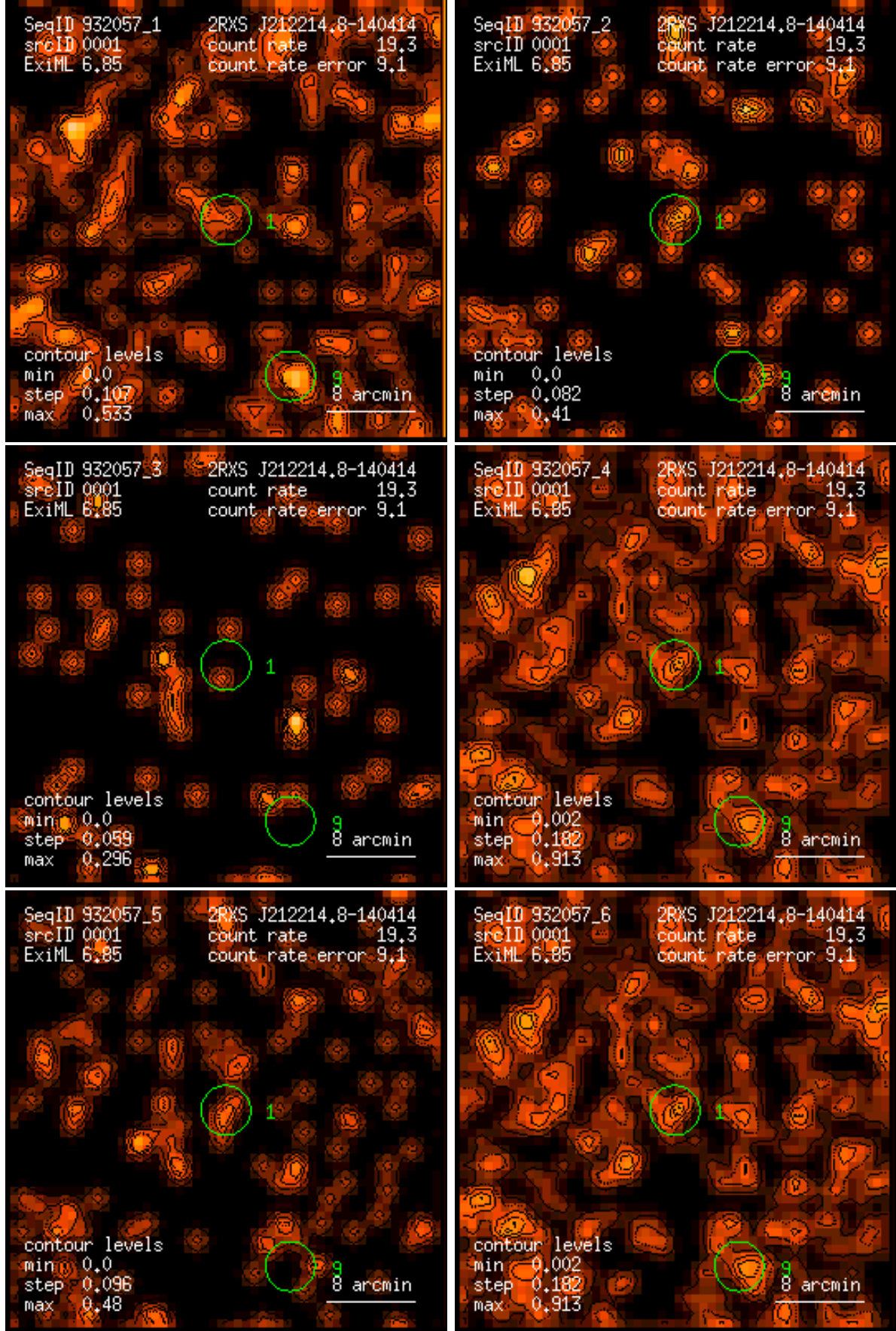
Figure 1: RASS 932057: detection 0001: band rate images, Gaussian filter: (1) PSPC channels 11 – 41, (2) 52 – 90, (3) 91 – 201, (4) 11 – 235, (5) 52 – 201, (6) 11 – 201. Broad band rates in counts/ks. Band rate contour levels in counts/ks/arcmin 2 .
