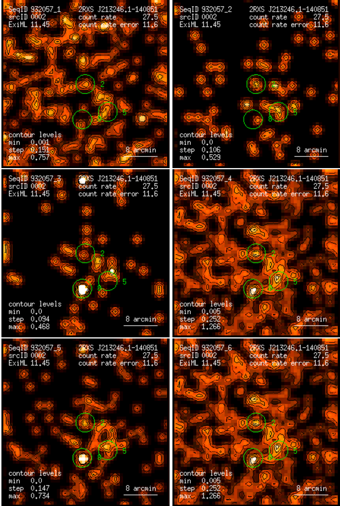
Figure 2: RASS 932057: detection 0002: band rate images, Gaussian filter: (1) PSPC channels 11 – 41, (2) 52 – 90, (3) 91 – 201, (4) 11 – 235, (5) 52 – 201, (6) 11 – 201. Broad band rates in counts/ks. Band rate contour levels in counts/ks/arcmin 2 .
