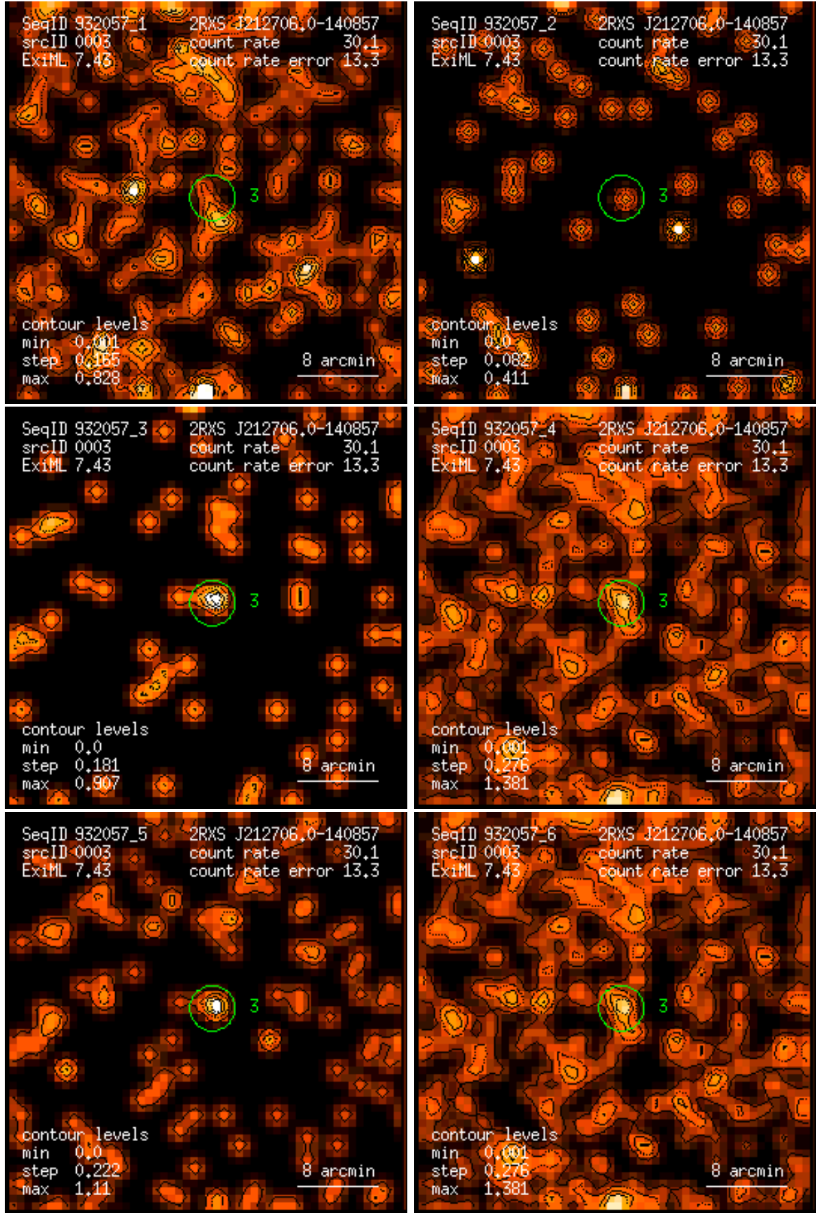
Figure 3: RASS 932057: detection 0003: band rate images, Gaussian filter: (1) PSPC channels 11 – 41, (2) 52 – 90, (3) 91 – 201, (4) 11 – 235, (5) 52 – 201, (6) 11 – 201. Broad band rates in counts/ks. Band rate contour levels in counts/ks/arcmin 2 .
