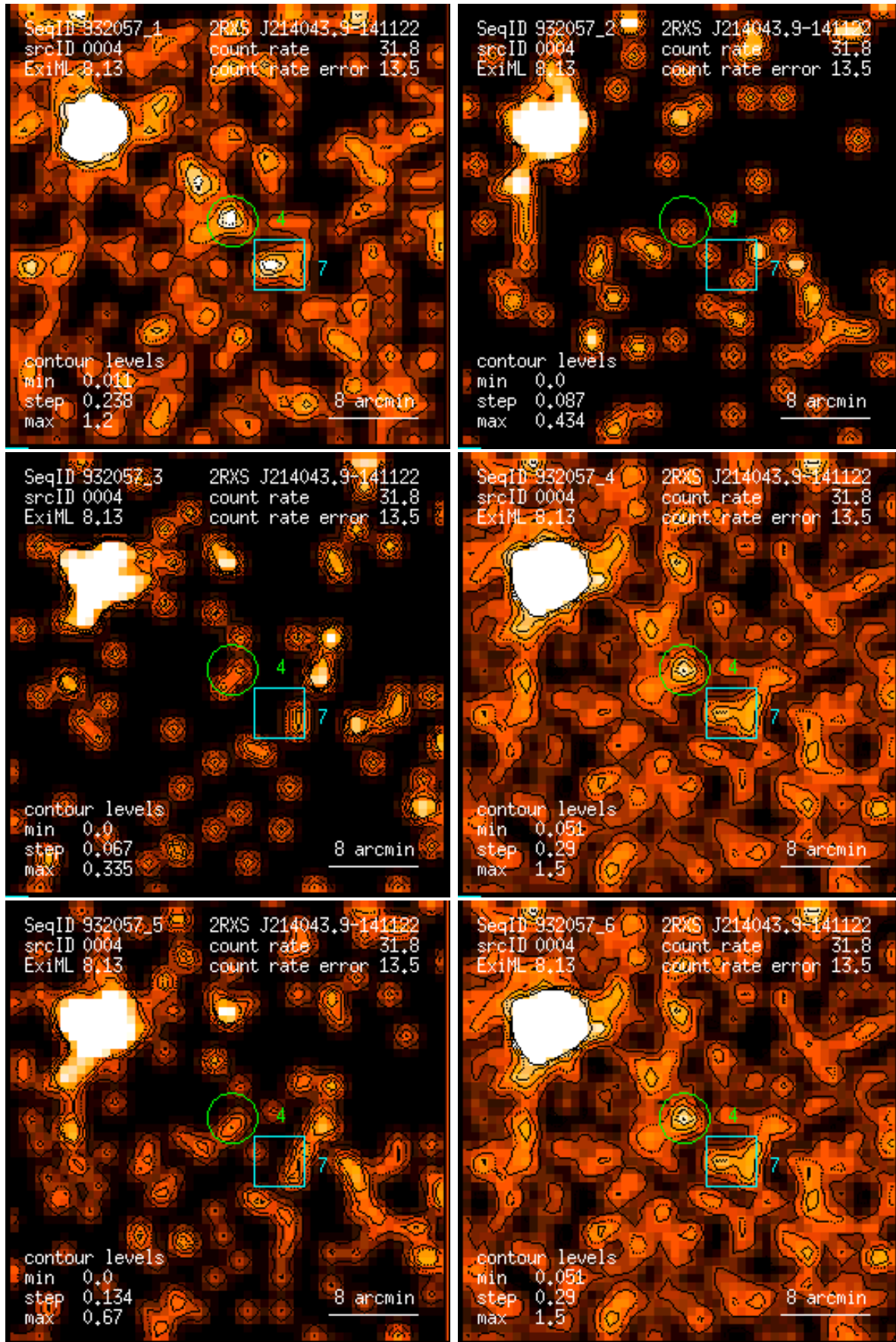
Figure 4: RASS 932057: detection 0004: band rate images, Gaussian filter: (1) PSPC channels 11 – 41, (2) 52 – 90, (3) 91 – 201, (4) 11 – 235, (5) 52 – 201, (6) 11 – 201. Broad band rates in counts/ks. Band rate contour levels in counts/ks/arcmin 2 .
