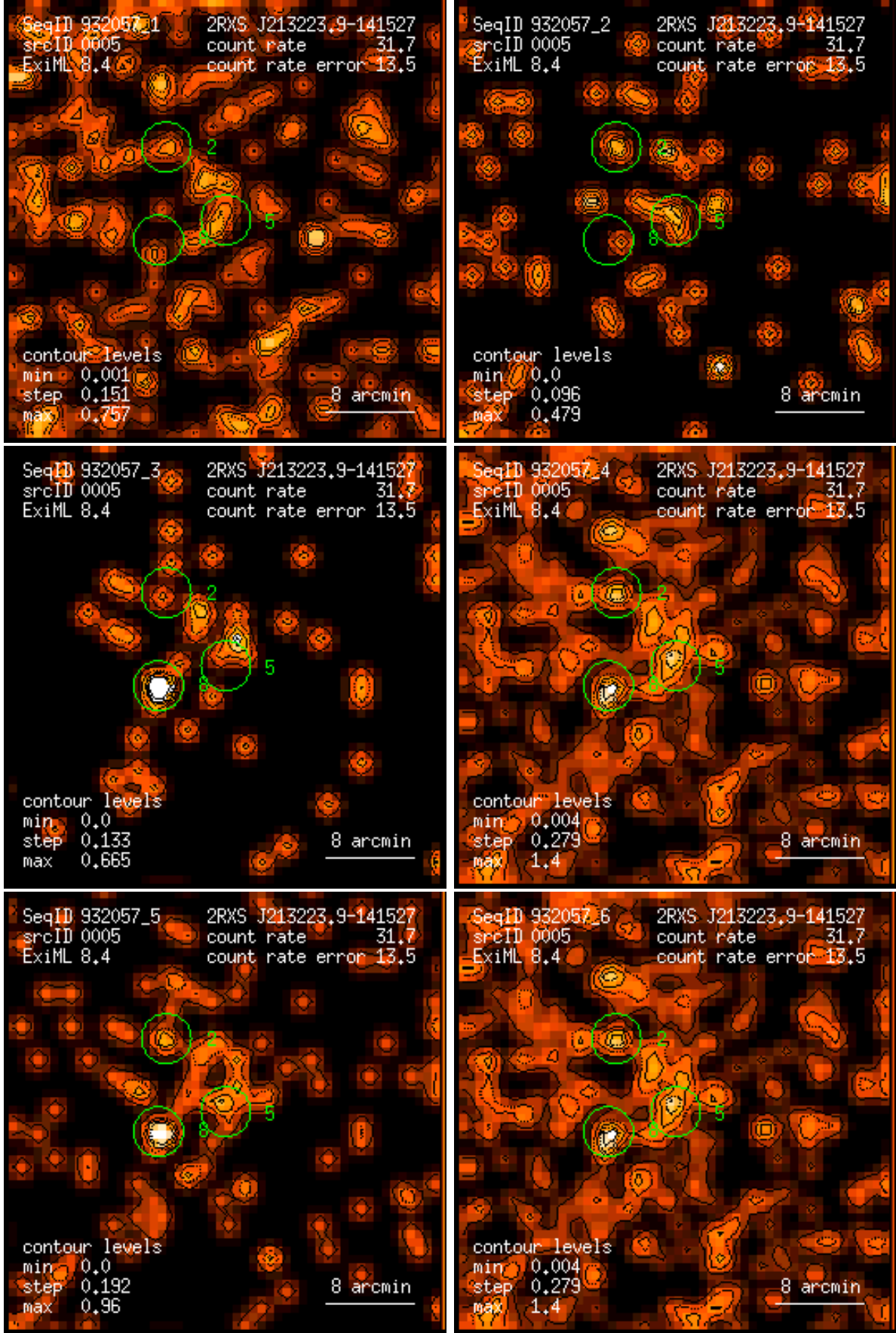
Figure 5: RASS 932057: detection 0005: band rate images, Gaussian filter: (1) PSPC channels 11 – 41, (2) 52 – 90, (3) 91 – 201, (4) 11 – 235, (5) 52 – 201, (6) 11 – 201. Broad band rates in counts/ks. Band rate contour levels in counts/ks/arcmin 2 .
