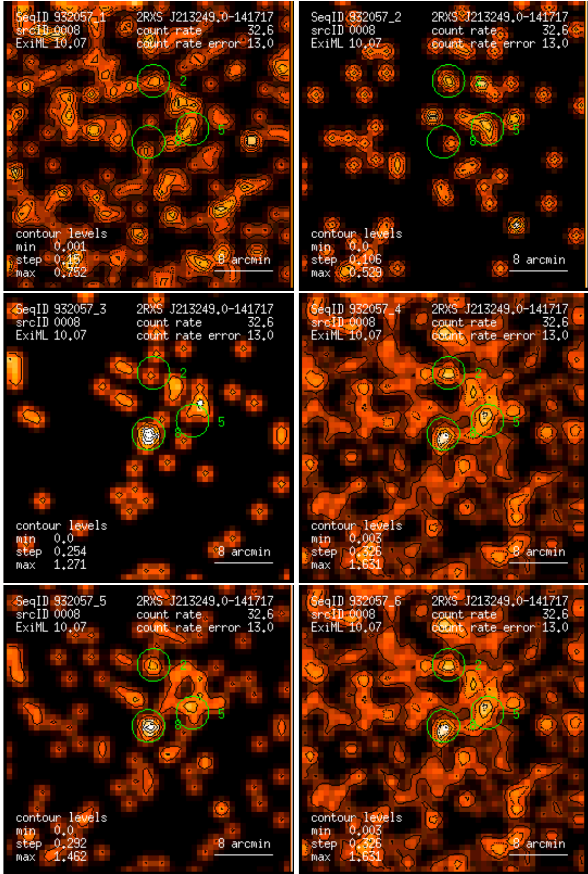
Figure 8: RASS 932057: detection 0008: band rate images, Gaussian filter: (1) PSPC channels 11 – 41, (2) 52 – 90, (3) 91 – 201, (4) 11 – 235, (5) 52 – 201, (6) 11 – 201. Broad band rates in counts/ks. Band rate contour levels in counts/ks/arcmin 2 .
