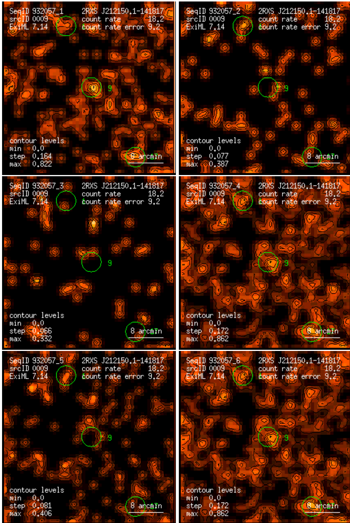
Figure 9: RASS 932057: detection 0009: band rate images, Gaussian filter: (1) PSPC channels 11 – 41, (2) 52 – 90, (3) 91 – 201, (4) 11 – 235, (5) 52 – 201, (6) 11 – 201. Broad band rates in counts/ks. Band rate contour levels in counts/ks/arcmin 2 .
