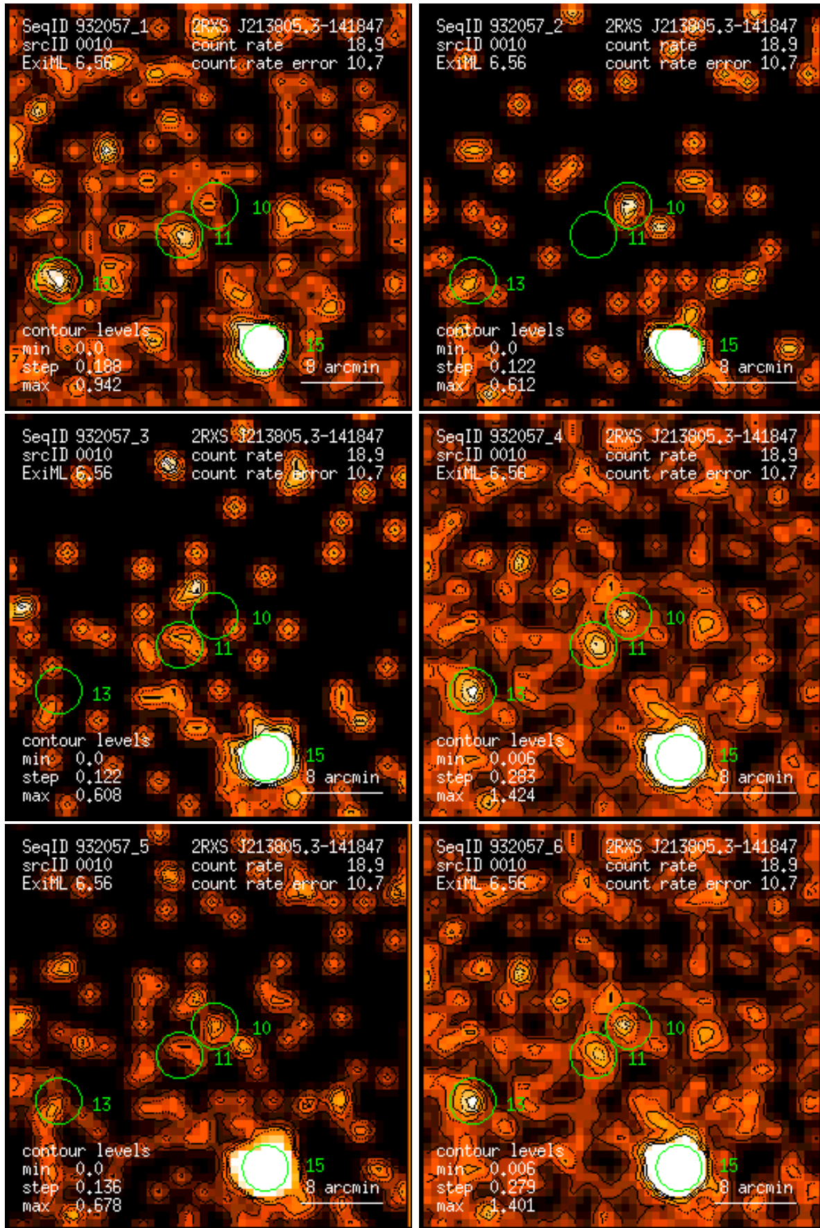
Figure 10: RASS 932057: detection 0010: band rate images, Gaussian filter: (1) PSPC channels 11 – 41, (2) 52 – 90, (3) 91 – 201, (4) 11 – 235, (5) 52 – 201, (6) 11 – 201. Broad band rates in counts/ks. Band rate contour levels in counts/ks/arcmin 2 .
