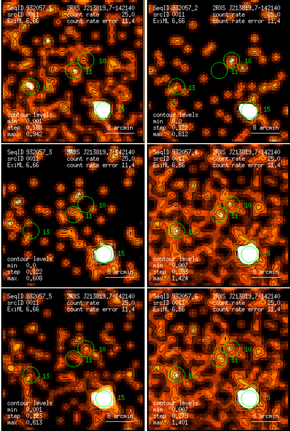
Figure 11: RASS 932057: detection 0011: band rate images, Gaussian filter: (1) PSPC channels 11 – 41, (2) 52 – 90, (3) 91 – 201, (4) 11 – 235, (5) 52 – 201, (6) 11 – 201. Broad band rates in counts/ks. Band rate contour levels in counts/ks/arcmin 2 .
