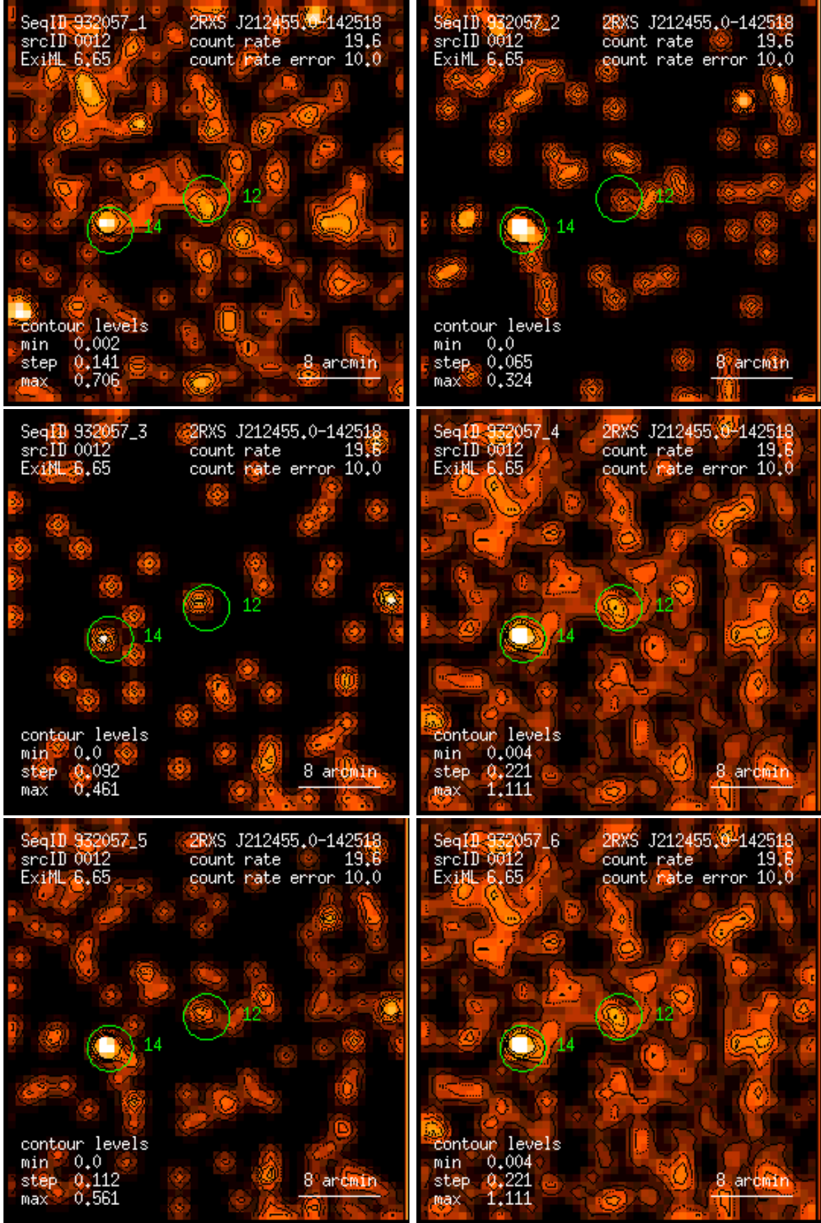
Figure 12: RASS 932057: detection 0012: band rate images, Gaussian filter: (1) PSPC channels 11 – 41, (2) 52 – 90, (3) 91 – 201, (4) 11 – 235, (5) 52 – 201, (6) 11 – 201. Broad band rates in counts/ks. Band rate contour levels in counts/ks/arcmin 2 .
