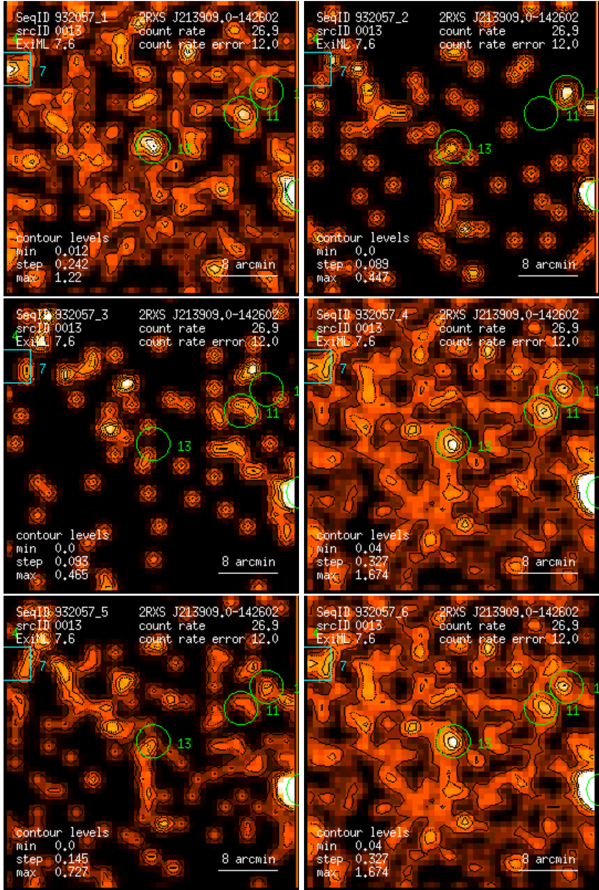
Figure 13: RASS 932057: detection 0013: band rate images, Gaussian filter: (1) PSPC channels 11 – 41, (2) 52 – 90, (3) 91 – 201, (4) 11 – 235, (5) 52 – 201, (6) 11 – 201. Broad band rates in counts/ks. Band rate contour levels in counts/ks/arcmin 2 .
