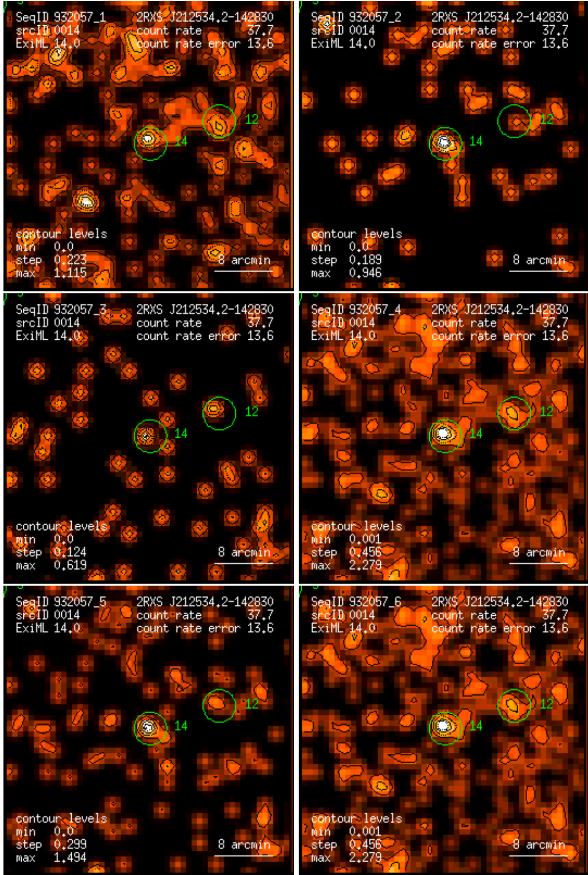
Figure 14: RASS 932057: detection 0014: band rate images, Gaussian filter: (1) PSPC channels 11 – 41, (2) 52 – 90, (3) 91 – 201, (4) 11 – 235, (5) 52 – 201, (6) 11 – 201. Broad band rates in counts/ks. Band rate contour levels in counts/ks/arcmin 2 .
