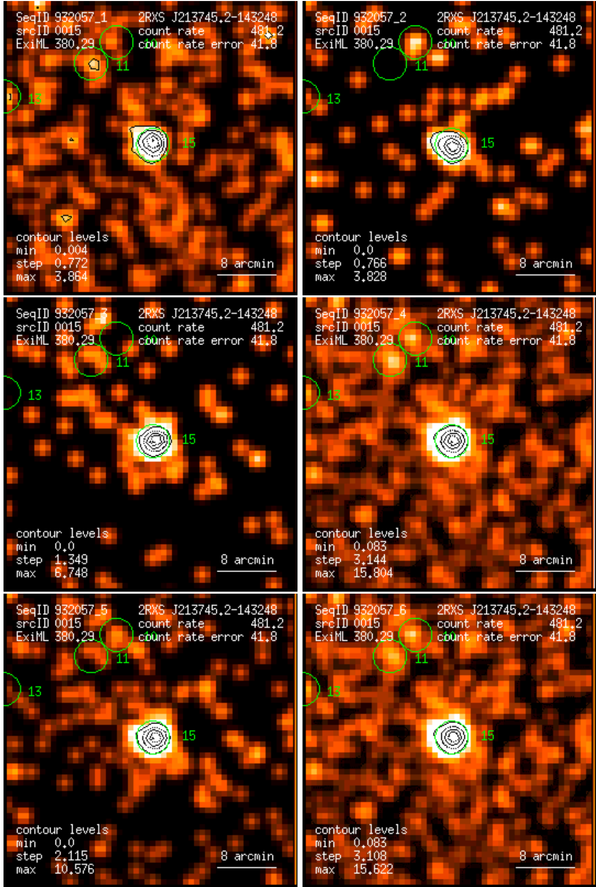
Figure 15: RASS 932057: detection 0015: band rate images, Gaussian filter: (1) PSPC channels 11 – 41, (2) 52 – 90, (3) 91 – 201, (4) 11 – 235, (5) 52 – 201, (6) 11 – 201. Broad band rates in counts/ks. Band rate contour levels in counts/ks/arcmin 2 .
