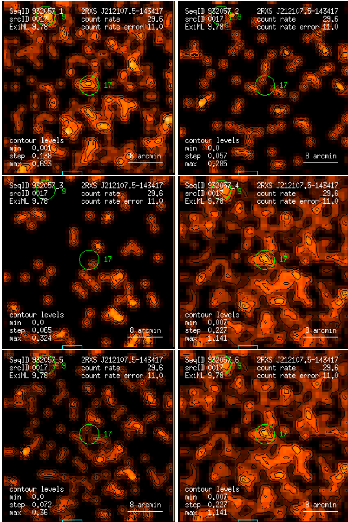
Figure 17: RASS 932057: detection 0017: band rate images, Gaussian filter: (1) PSPC channels 11 – 41, (2) 52 – 90, (3) 91 – 201, (4) 11 – 235, (5) 52 – 201, (6) 11 – 201. Broad band rates in counts/ks. Band rate contour levels in counts/ks/arcmin 2 .
