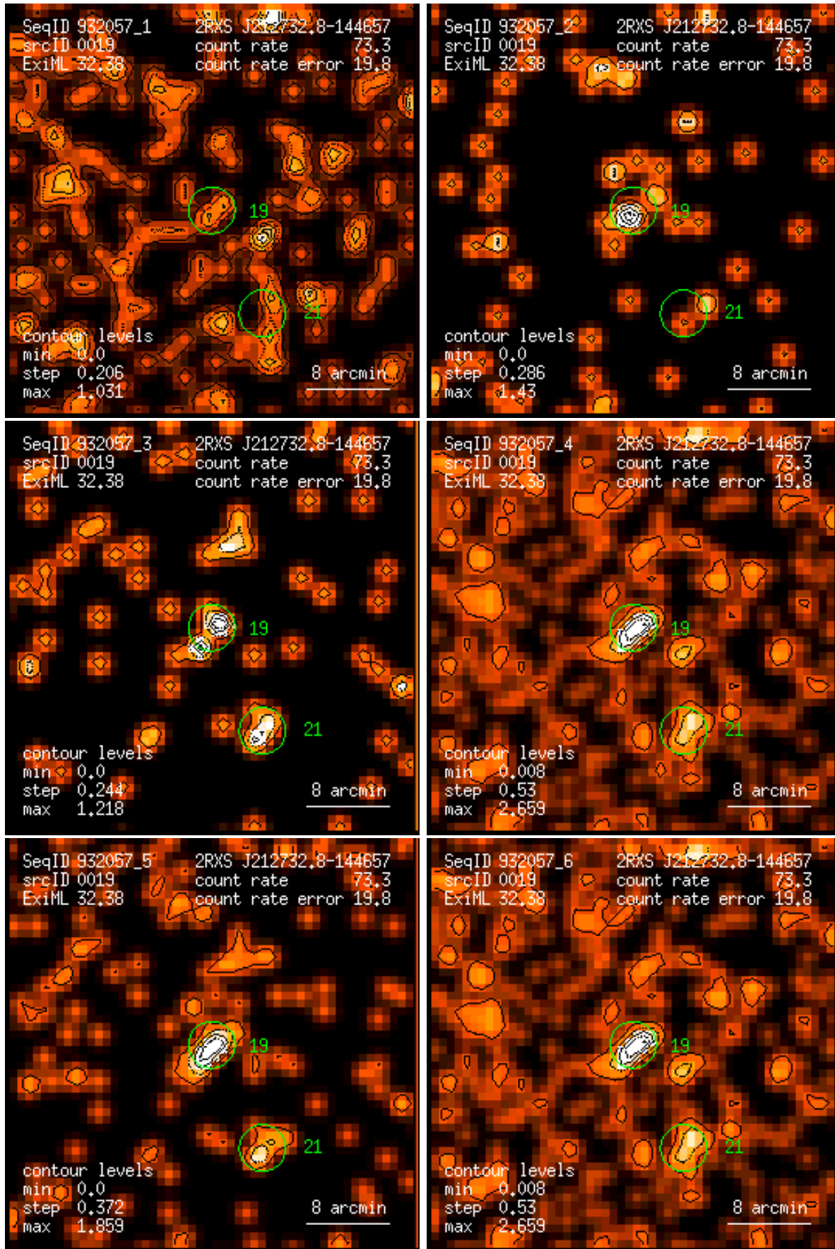
Figure 19: RASS 932057: detection 0019: band rate images, Gaussian filter: (1) PSPC channels 11 – 41, (2) 52 – 90, (3) 91 – 201, (4) 11 – 235, (5) 52 – 201, (6) 11 – 201. Broad band rates in counts/ks. Band rate contour levels in counts/ks/arcmin 2 .
