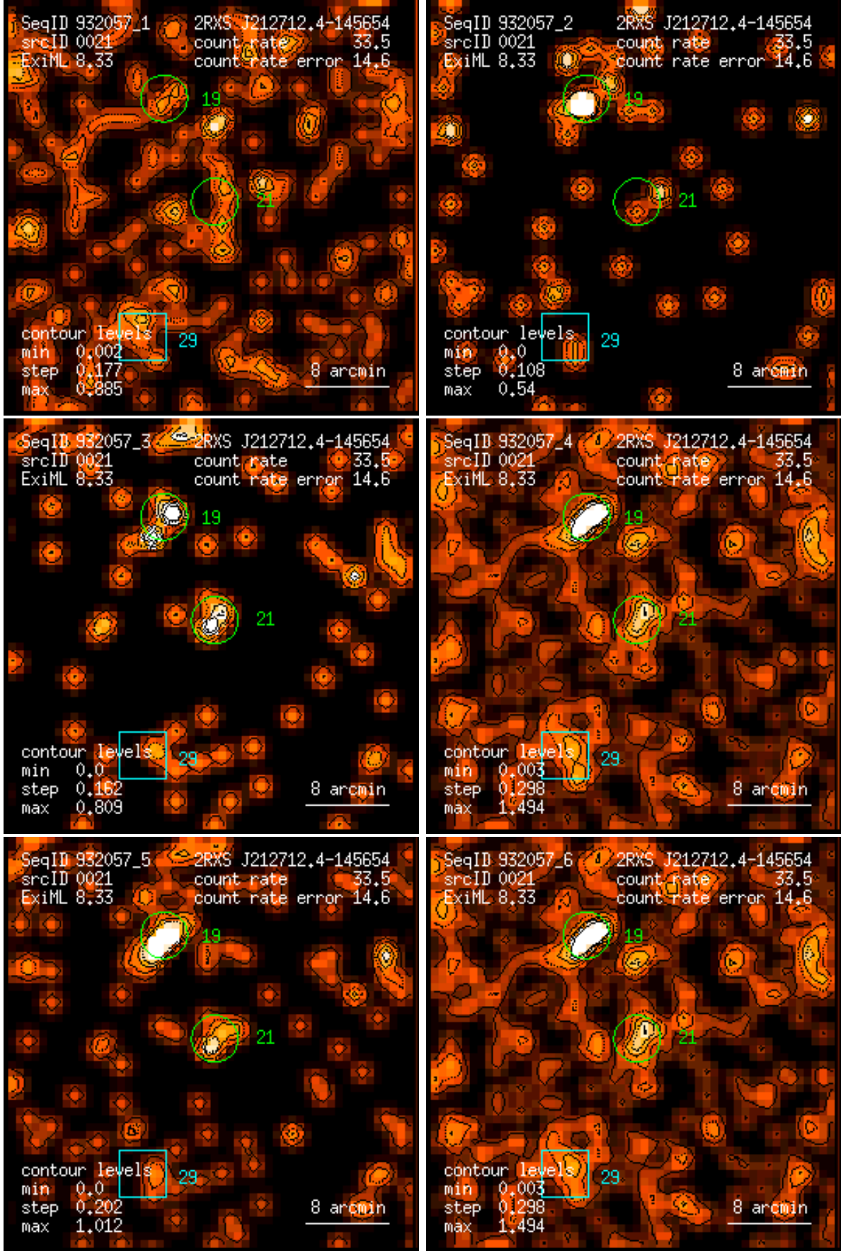
Figure 21: RASS 932057: detection 0021: band rate images, Gaussian filter: (1) PSPC channels 11 – 41, (2) 52 – 90, (3) 91 – 201, (4) 11 – 235, (5) 52 – 201, (6) 11 – 201. Broad band rates in counts/ks. Band rate contour levels in counts/ks/arcmin 2 .
