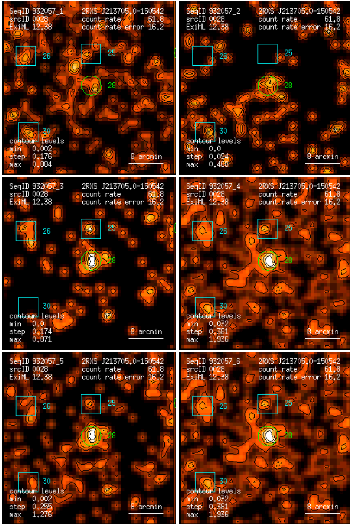
Figure 28: RASS 932057: detection 0028: band rate images, Gaussian filter: (1) PSPC channels 11 – 41, (2) 52 – 90, (3) 91 – 201, (4) 11 – 235, (5) 52 – 201, (6) 11 – 201. Broad band rates in counts/ks. Band rate contour levels in counts/ks/arcmin 2 .
