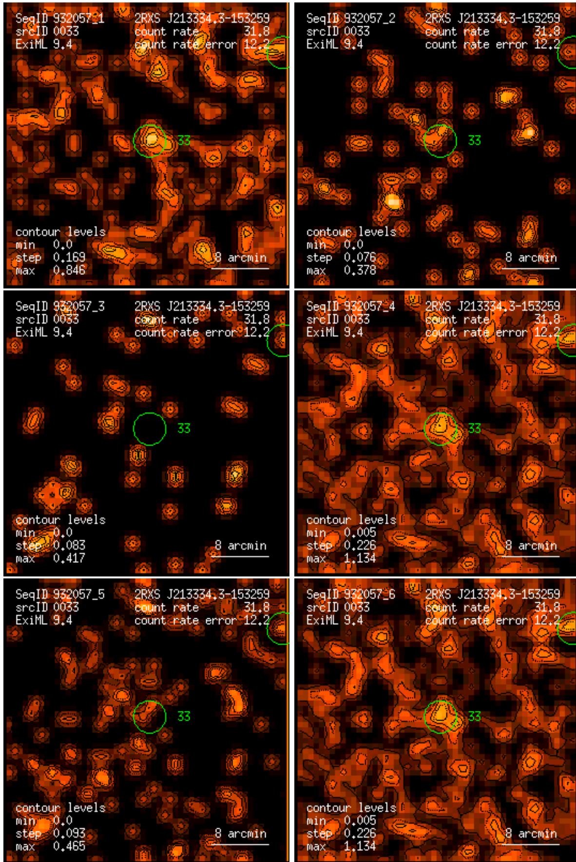
Figure 33: RASS 932057: detection 0033: band rate images, Gaussian filter: (1) PSPC channels 11 – 41, (2) 52 – 90, (3) 91 – 201, (4) 11 – 235, (5) 52 – 201, (6) 11 – 201. Broad band rates in counts/ks. Band rate contour levels in counts/ks/arcmin 2 .
