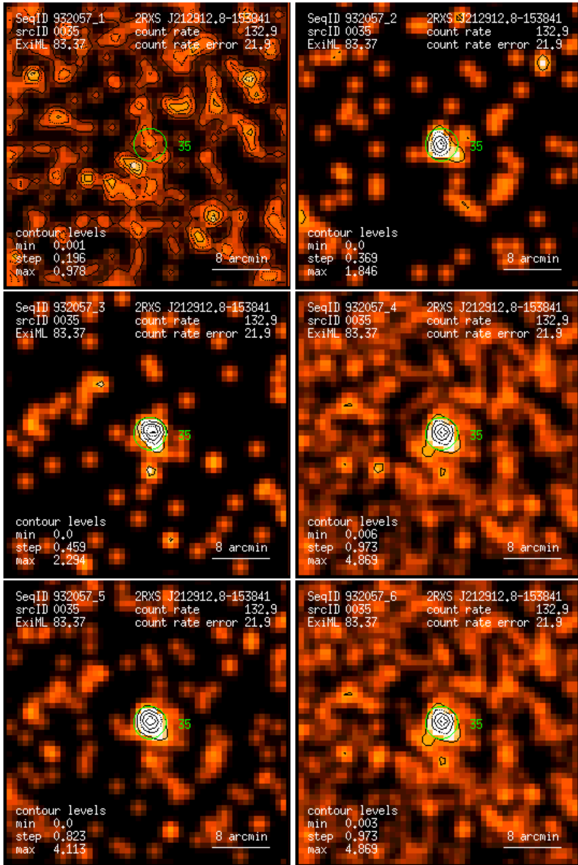
Figure 35: RASS 932057: detection 0035: band rate images, Gaussian filter: (1) PSPC channels 11 – 41, (2) 52 – 90, (3) 91 – 201, (4) 11 – 235, (5) 52 – 201, (6) 11 – 201. Broad band rates in counts/ks. Band rate contour levels in counts/ks/arcmin 2 .
