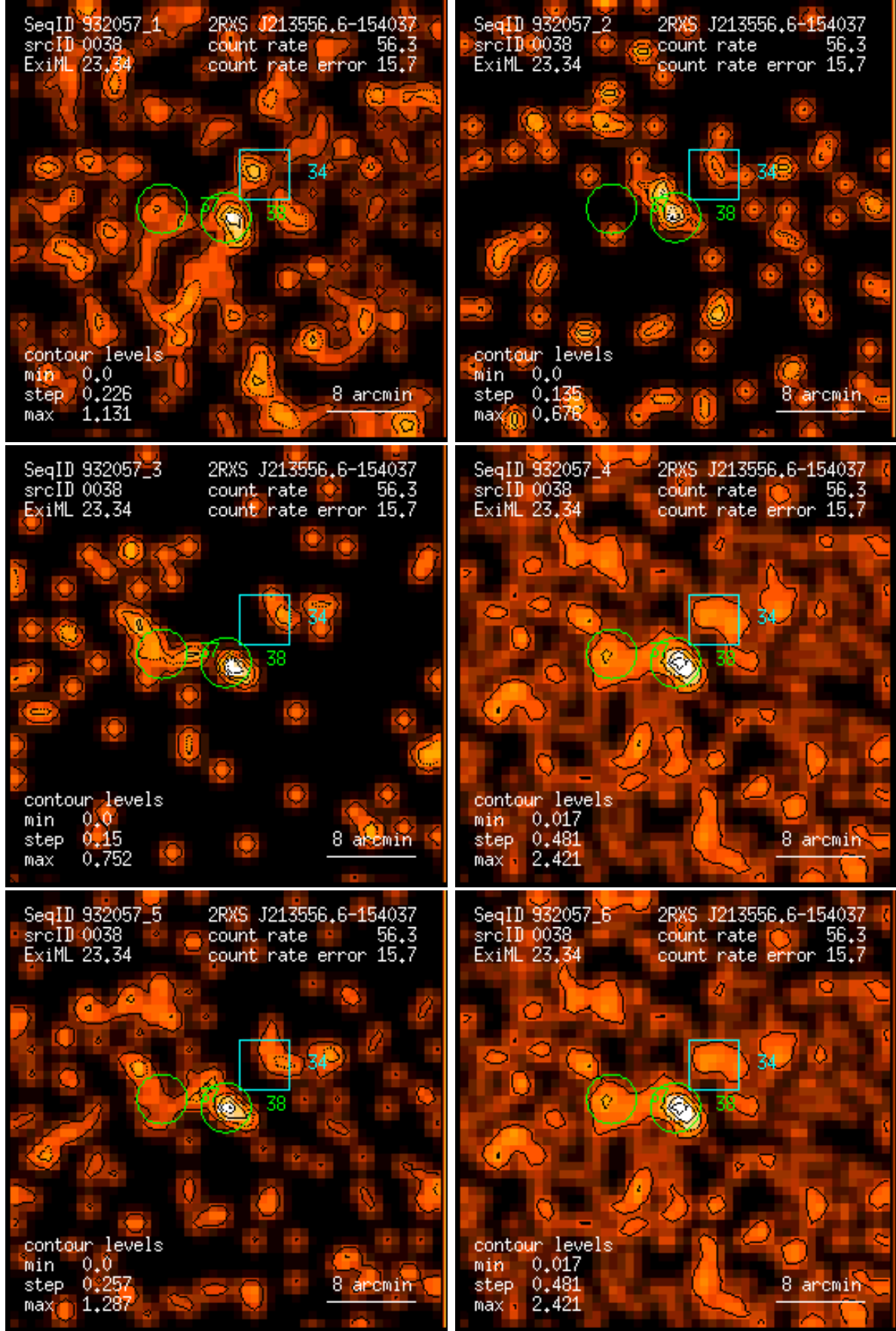
Figure 38: RASS 932057: detection 0038: band rate images, Gaussian filter: (1) PSPC channels 11 – 41, (2) 52 – 90, (3) 91 – 201, (4) 11 – 235, (5) 52 – 201, (6) 11 – 201. Broad band rates in counts/ks. Band rate contour levels in counts/ks/arcmin 2 .
