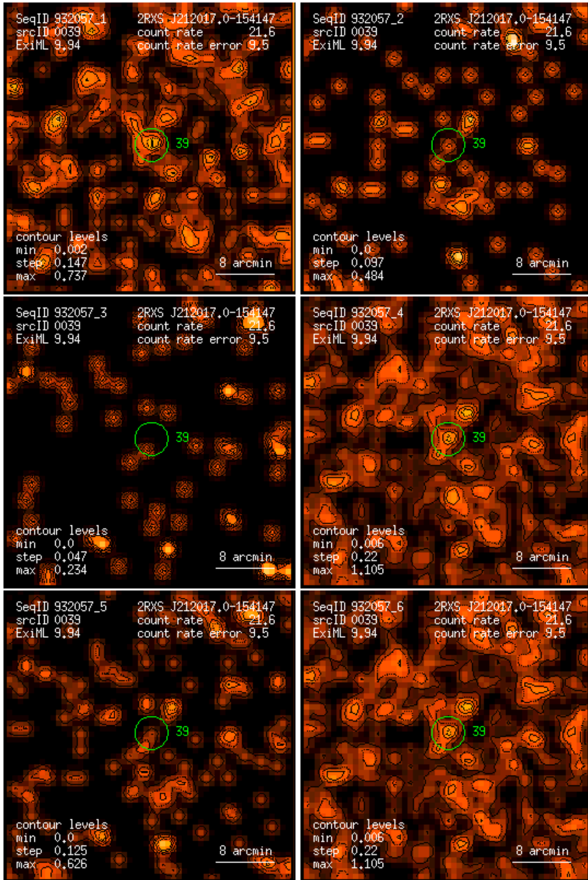
Figure 39: RASS 932057: detection 0039: band rate images, Gaussian filter: (1) PSPC channels 11 – 41, (2) 52 – 90, (3) 91 – 201, (4) 11 – 235, (5) 52 – 201, (6) 11 – 201. Broad band rates in counts/ks. Band rate contour levels in counts/ks/arcmin 2 .
