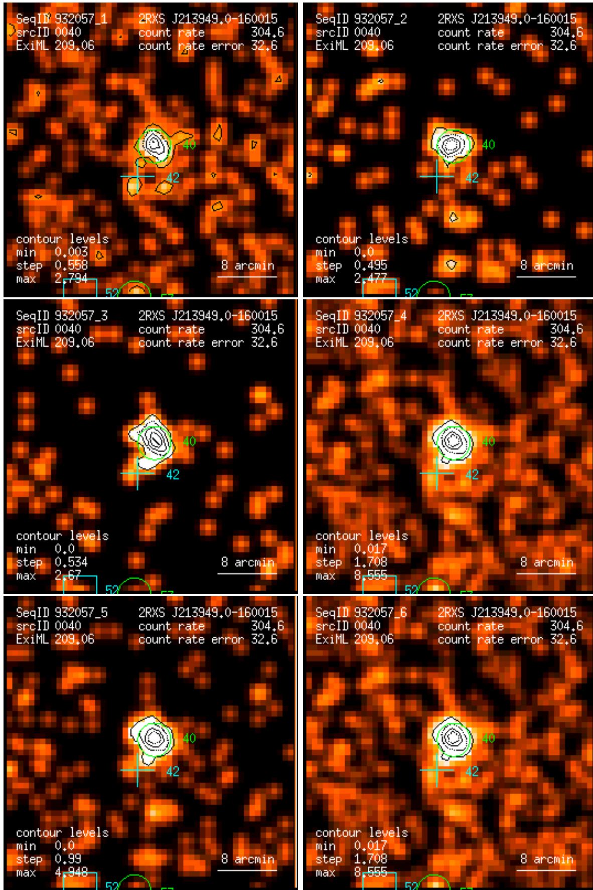
Figure 40: RASS 932057: detection 0040: band rate images, Gaussian filter: (1) PSPC channels 11 – 41, (2) 52 – 90, (3) 91 – 201, (4) 11 – 235, (5) 52 – 201, (6) 11 – 201. Broad band rates in counts/ks. Band rate contour levels in counts/ks/arcmin 2 .
