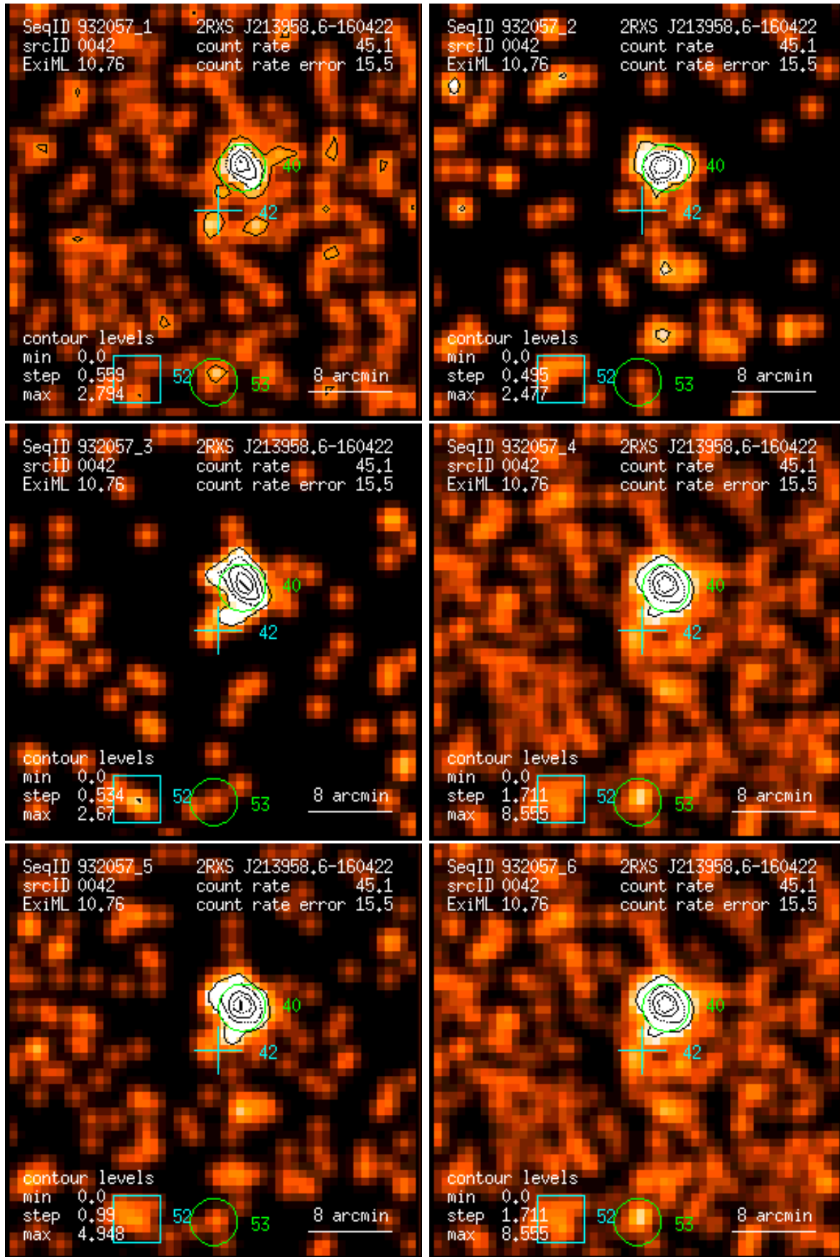
Figure 42: RASS 932057: detection 0042: band rate images, Gaussian filter: (1) PSPC channels 11 – 41, (2) 52 – 90, (3) 91 – 201, (4) 11 – 235, (5) 52 – 201, (6) 11 – 201. Broad band rates in counts/ks. Band rate contour levels in counts/ks/arcmin 2 .
