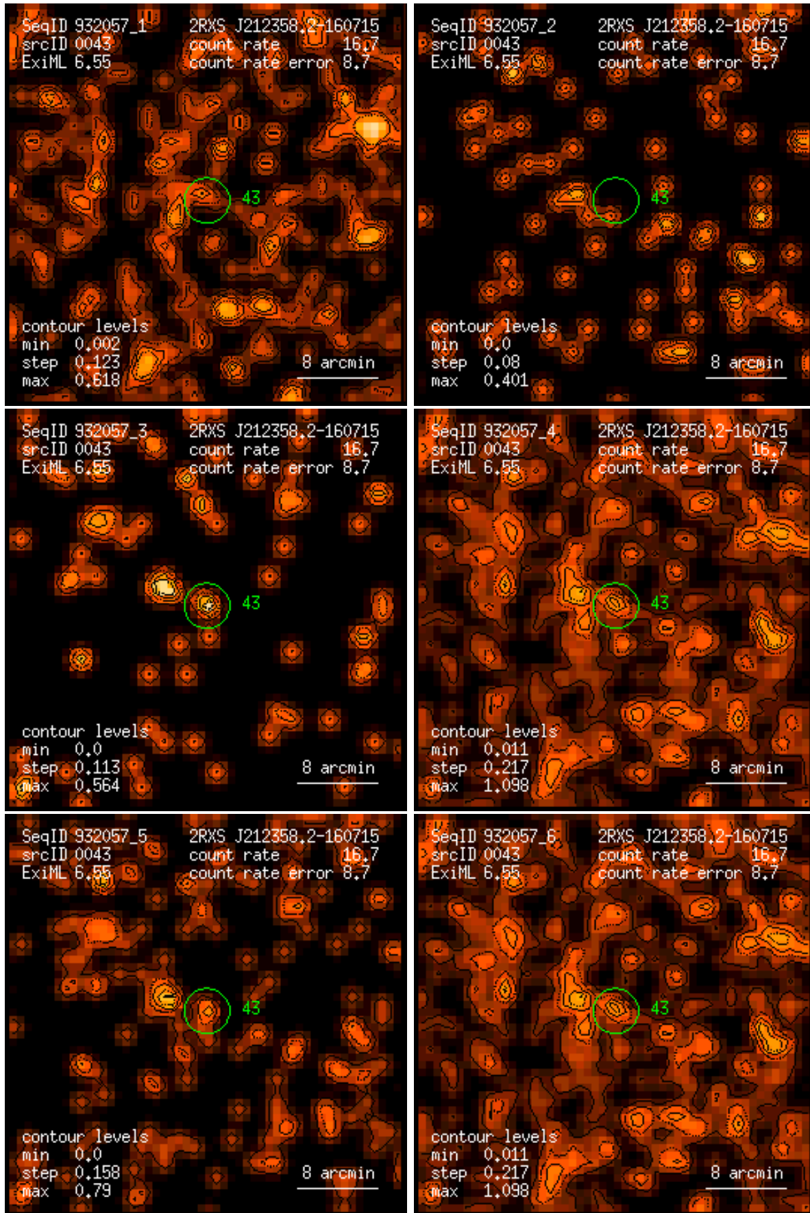
Figure 43: RASS 932057: detection 0043: band rate images, Gaussian filter: (1) PSPC channels 11 – 41, (2) 52 – 90, (3) 91 – 201, (4) 11 – 235, (5) 52 – 201, (6) 11 – 201. Broad band rates in counts/ks. Band rate contour levels in counts/ks/arcmin 2 .
