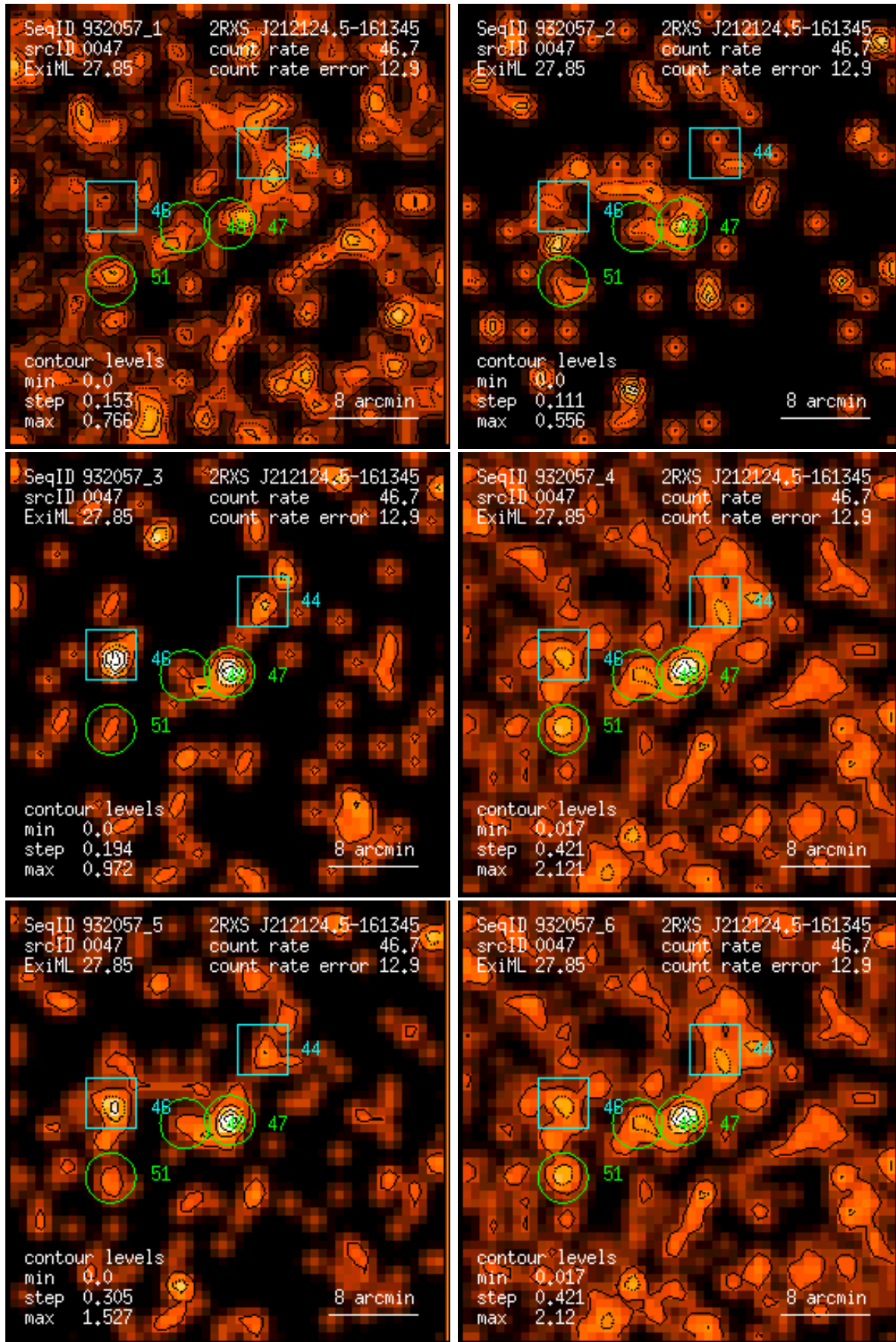
Figure 47: RASS 932057: detection 0047: band rate images, Gaussian filter: (1) PSPC channels 11 – 41, (2) 52 – 90, (3) 91 – 201, (4) 11 – 235, (5) 52 – 201, (6) 11 – 201. Broad band rates in counts/ks. Band rate contour levels in counts/ks/arcmin 2 .
