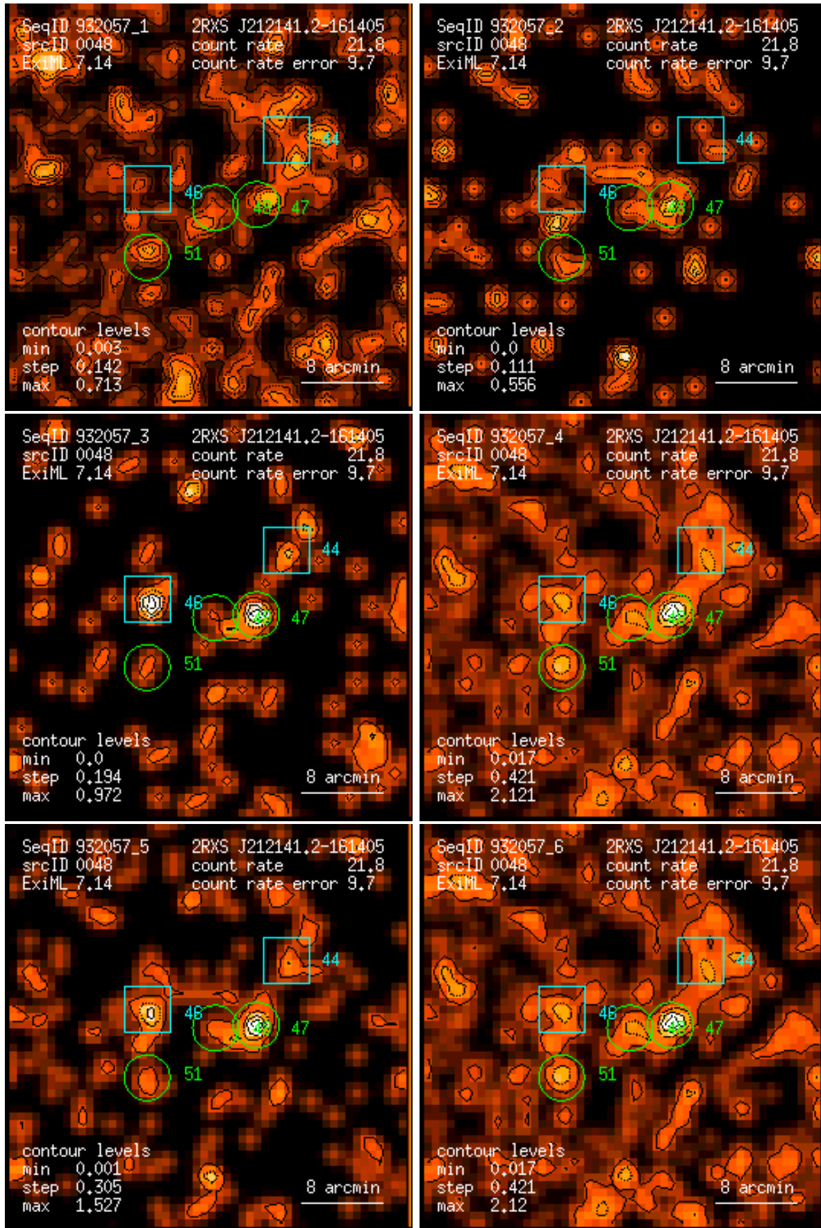
Figure 48: RASS 932057: detection 0048: band rate images, Gaussian filter: (1) PSPC channels 11 – 41, (2) 52 – 90, (3) 91 – 201, (4) 11 – 235, (5) 52 – 201, (6) 11 – 201. Broad band rates in counts/ks. Band rate contour levels in counts/ks/arcmin 2 .
