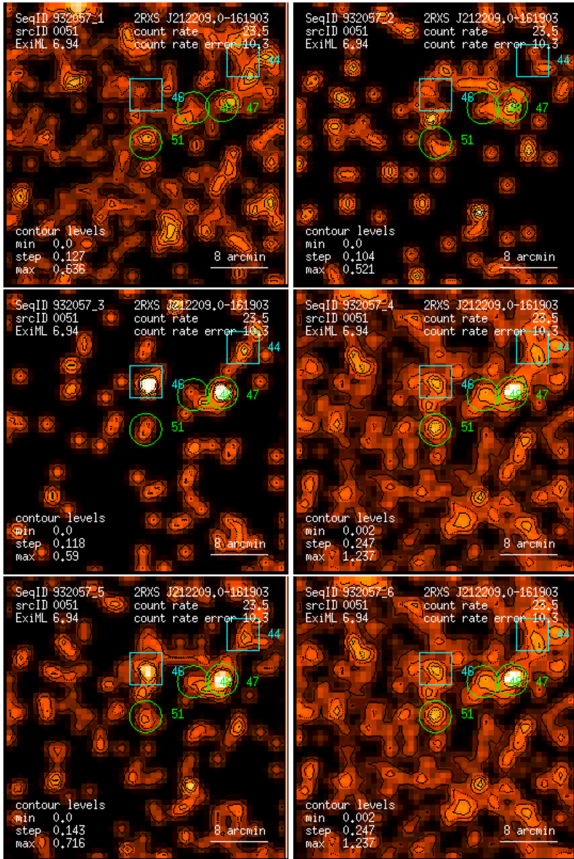
Figure 51: RASS 932057: detection 0051: band rate images, Gaussian filter: (1) PSPC channels 11 – 41, (2) 52 – 90, (3) 91 – 201, (4) 11 – 235, (5) 52 – 201, (6) 11 – 201. Broad band rates in counts/ks. Band rate contour levels in counts/ks/arcmin 2 .
