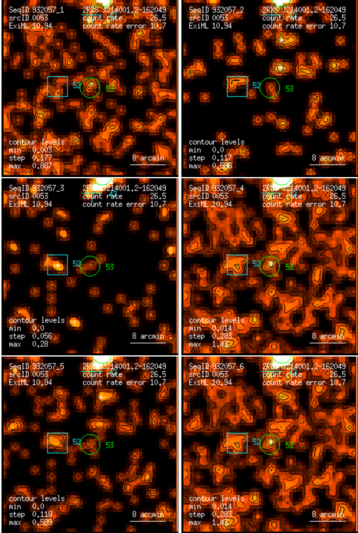
Figure 53: RASS 932057: detection 0053: band rate images, Gaussian filter: (1) PSPC channels 11 – 41, (2) 52 – 90, (3) 91 – 201, (4) 11 – 235, (5) 52 – 201, (6) 11 – 201. Broad band rates in counts/ks. Band rate contour levels in counts/ks/arcmin 2 .
