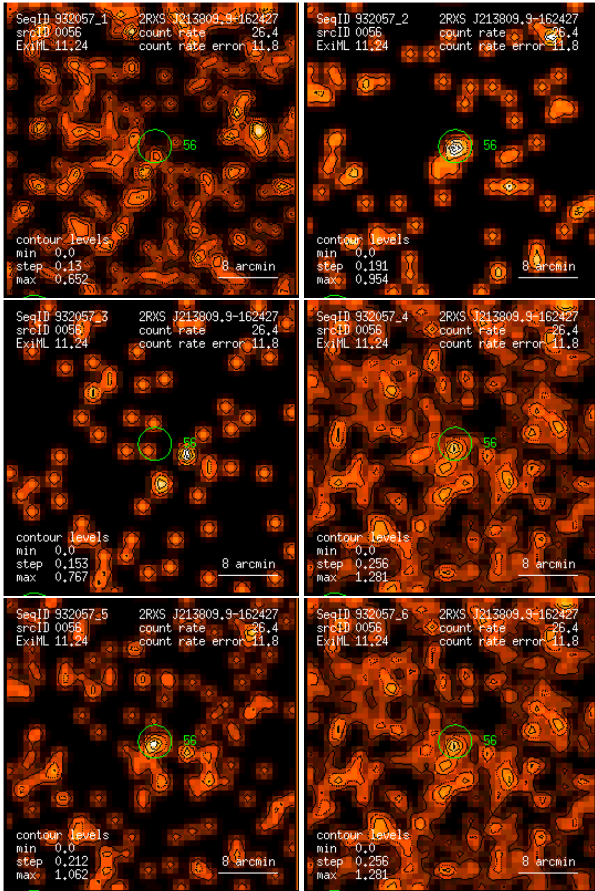
Figure 56: RASS 932057: detection 0056: band rate images, Gaussian filter: (1) PSPC channels 11 – 41, (2) 52 – 90, (3) 91 – 201, (4) 11 – 235, (5) 52 – 201, (6) 11 – 201. Broad band rates in counts/ks. Band rate contour levels in counts/ks/arcmin 2 .
