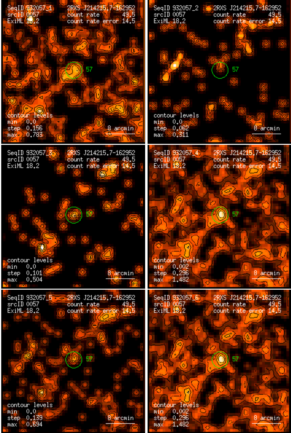
Figure 57: RASS 932057: detection 0057: band rate images, Gaussian filter: (1) PSPC channels 11 – 41, (2) 52 – 90, (3) 91 – 201, (4) 11 – 235, (5) 52 – 201, (6) 11 – 201. Broad band rates in counts/ks. Band rate contour levels in counts/ks/arcmin 2 .
